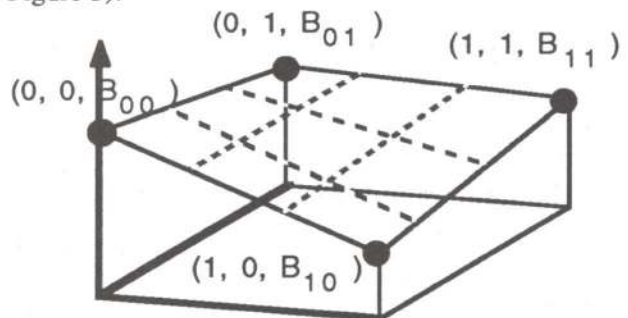
Figure 5. Bilinear interpolation.
