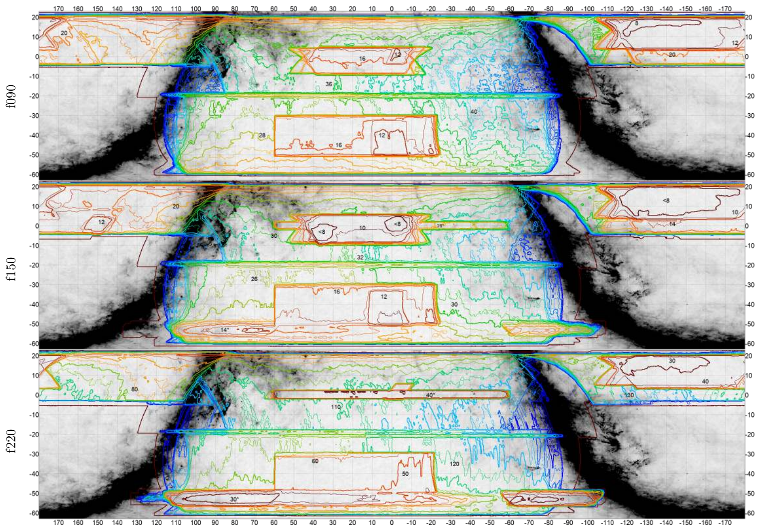
Figure 15: Spatial distribution of ACT-only map depths for the three different ACT frequencies, as shown by iso-depth contours that go from 8/8/30 \mu\text{K}\text{-arcmin} (red) to 60/50/180 \mu\text{K}\text{-arcmin} (blue) with contour intervals of 2/2/10 \mu\text{K}\text{-arcmin} for f090/f150/f220 respectively. This covers most of the depth range in the maps, though there are areas that are somewhat deeper or shallower. The outermost red curve shows the full outline of the survey area. Selected contour lines are labeled with their depth to make it easier to read off values. These are T noise levels; Q and U are approximately \sqrt{2} higher. They also only describe the noise level at small scales. The background grayscale map is the dust-dominated Planck 353 GHz map.
