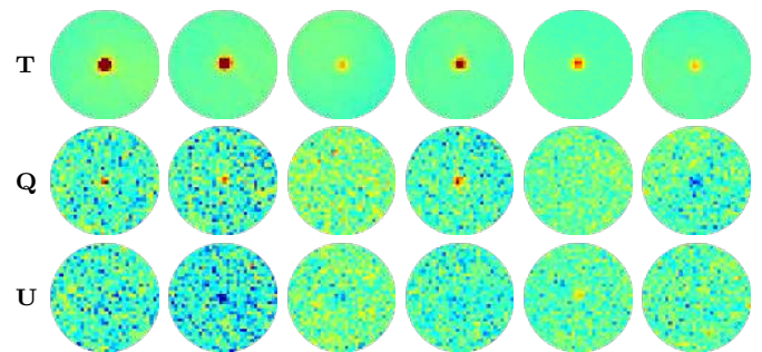
FIG. 15.— Three of the highest signal-to-noise polarized point sources from each of patch D5 (left) and D6 (right). Each disk has a radius of 8' , with the value range being \pm 2000 \mu\text{K} for T and \pm 200 \mu\text{K} for Q and U. We do not mask polarized sources in this analysis. The sources may be associated with (from left to right) [HB89] 2332-017, [HB89] 2335-027, SDSS J001130.40+005751.7, PKS 0214-085, [HB89] 0226-038 and PKS 0205-010.
