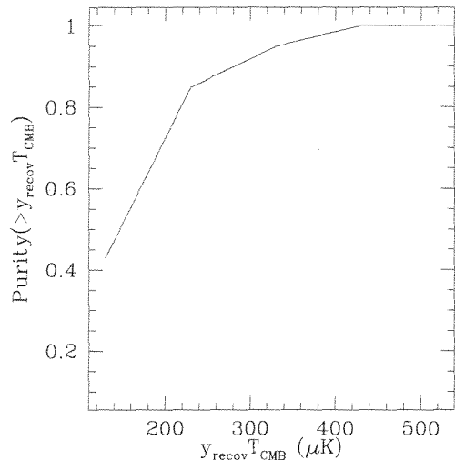
FIG. 4.— Purity versus recovered yT_{\text{CMB}} from simulations. For an observed yT_{\text{CMB}} threshold of 300 \mu\text{K} we expect our sample to be about 90% pure. Our actual sample is 100% pure, as each candidate cluster has been confirmed by optical observations (Menanteau et al. 2010a).
