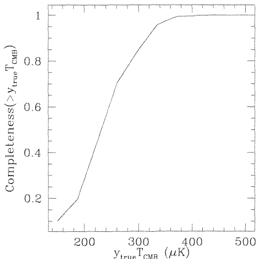
FIG. 3.— Completeness versus true yT_{\text{CMB}} from simulations. For an observed yT_{\text{CMB}} threshold of 300 \mu\text{K} we expect our sample to be about 85% complete for true yT_{\text{CMB}} values above 300 \mu\text{K} .
