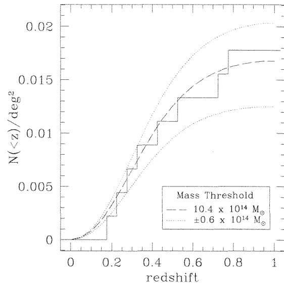
FIG. 2.— The redshift distribution of the 9 high-significance clusters listed in Table 1 compared to expectations from the mass function of Tinker et al. (2008) assuming all clusters above a given mass threshold have been detected. Here we assume the total area observed is 455 square degrees with uniform coverage, and the WMAP7+BAO+SN best-fit cosmology for a \Lambda CDM model (Komatsu et al. 2010) for the mass function. This figure suggests an effective mass threshold of our sample of \approx 10.4 \times 10^{14} M_{\odot} (dashed line). For illustrative purposes we show via dotted lines the expected redshift distributions for mass thresholds larger/smaller by 0.6 \times 10^{14} M_{\odot} .
