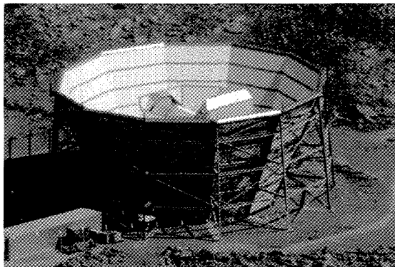
FIG. 1.— Picture ( left ) and mechanical rendering ( right ) of ACT and its ground screens. The telescope has a low profile; the full height is 12 m. The entire upper structure (“Azimuth structure” and above) rotates as a unit. The surrounding outer ground screen shields the telescope from ground emission. The screen also acts as a wind shield. An inner ground screen mounted on the telescope connects the sides of the secondary and primary. The primary reflector is 6 m and is surrounded by a 0.5 m guard ring (Figures courtesy of AMEC Dynamic Structures).
