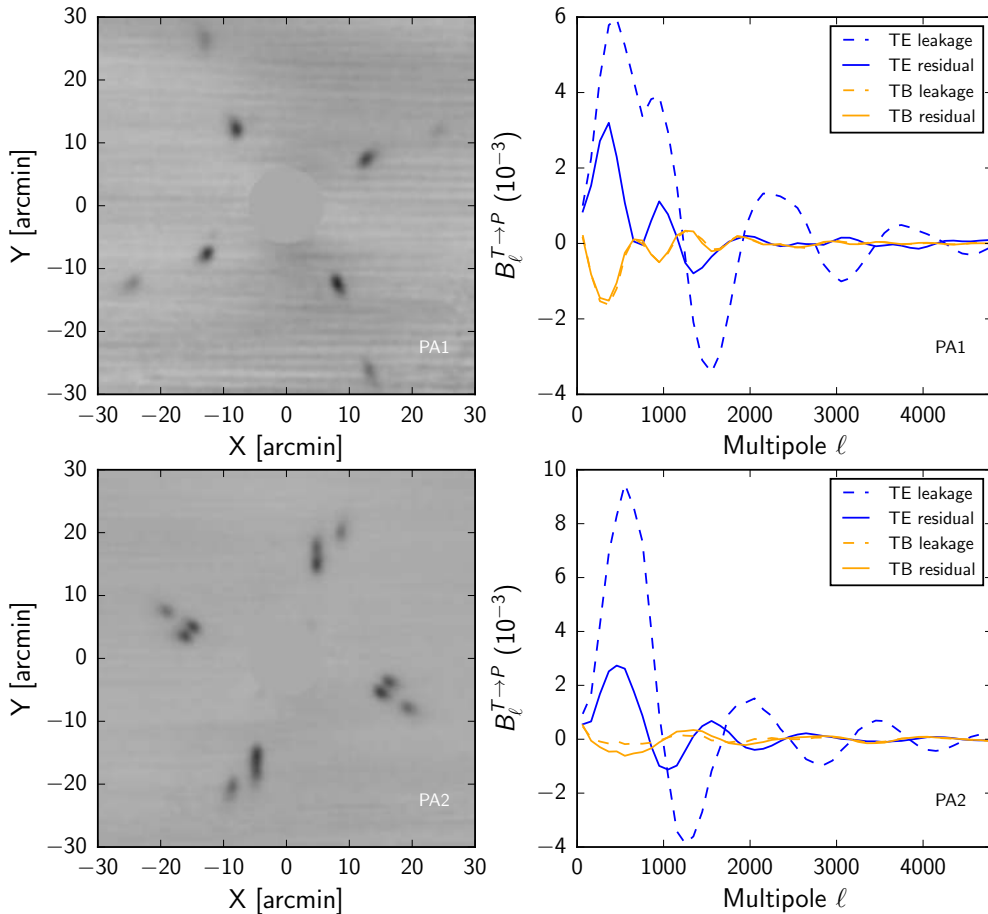
FIG. 4.— Polarized sidelobes in PA1 (top row) and PA2 (bottom row). Left panels show maps of the beam sidelobes, from 20 observations of Saturn. Spatial coordinates are relative to the main beam, which is masked here. Grayscale provides the sidelobe amplitude in the range -0.002 (black) to +0.001 (white) relative to the main beam peak, with negative signal indicating polarization perpendicular to the ray from the origin. The complementary polarization component (corresponding to TB leakage) is smaller and not shown in the maps but is included in the evaluation of the transfer functions. Right panels show the TE and TB transfer functions, normalized in units of the main beam, as in Figure 3, before and after the sidelobe deprojection procedure.
