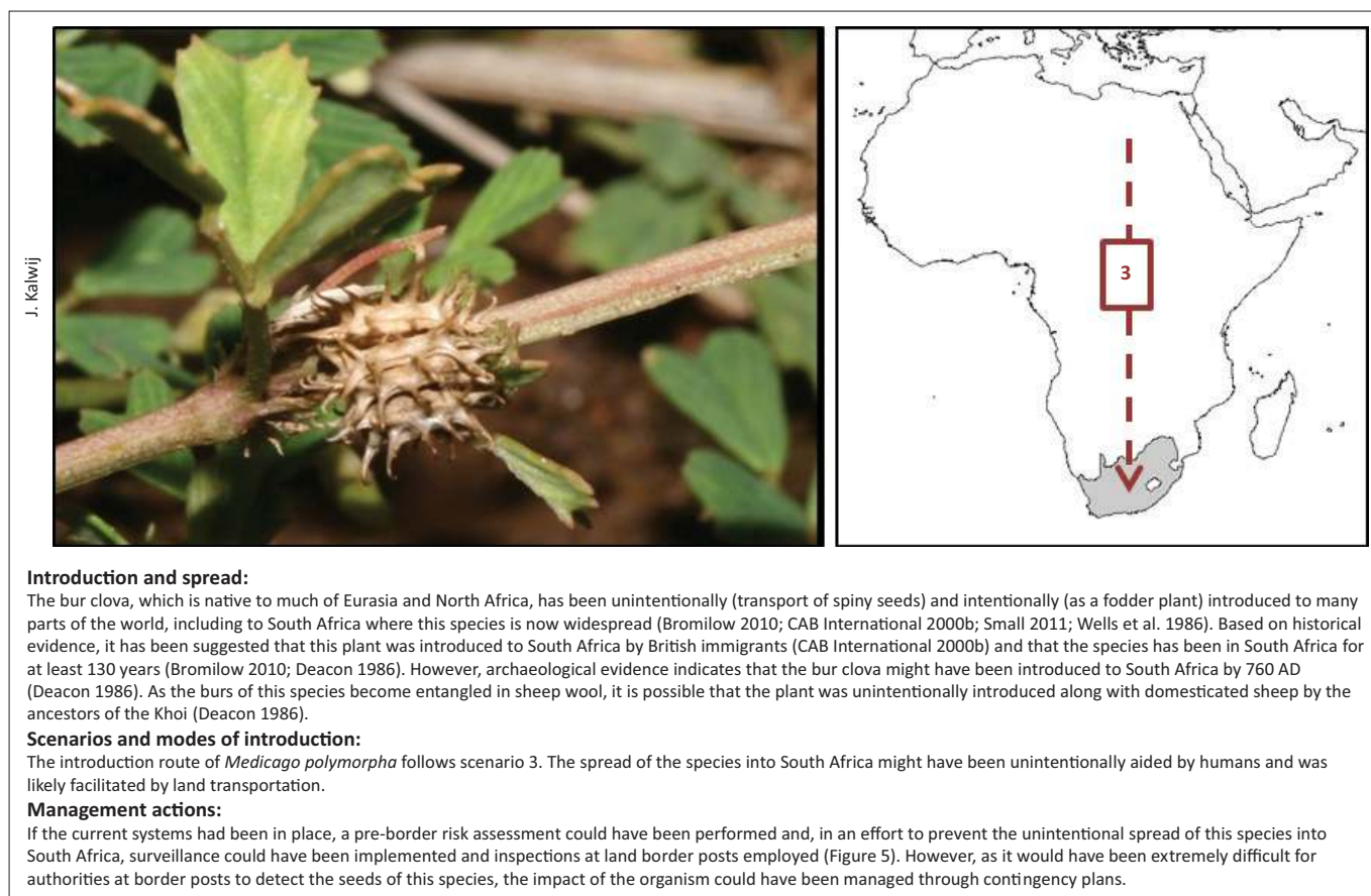
FIGURE 3-A2: Details on the introduction and spread of Medicago polymorpha , the relevant introduction route scenario and modes of transport, and the management actions that could have prevented or mitigated the invasion.
