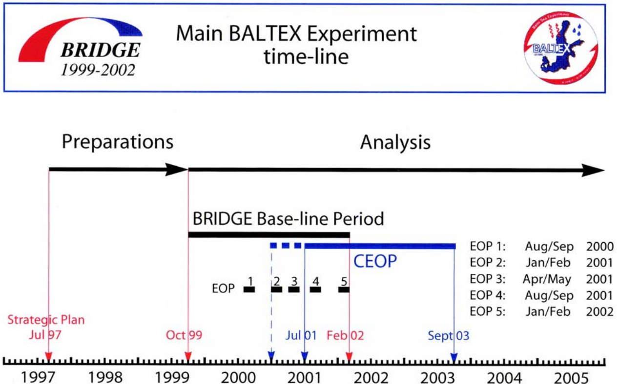
FIG. 2. Major activities within the BALTEX. Enhanced Observing Periods (EOPs) are defined to concentrate on specific process-oriented studies. CEOP is the Coordinated Enhanced Observational Period of all CSEs.
