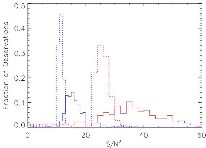
Figure 5. Fraction of completed plates as a function of S/N^2 as reported by SOS. The S/N^2 for the first year of data is shown as a solid line while the S/N^2 for the simulated survey, with somewhat lower thresholds as described in Section 5.5, is shown as the broken line. In both cases, the S/N^2 for the red cameras is shown in red while the S/N^2 for blue cameras is shown in blue.
