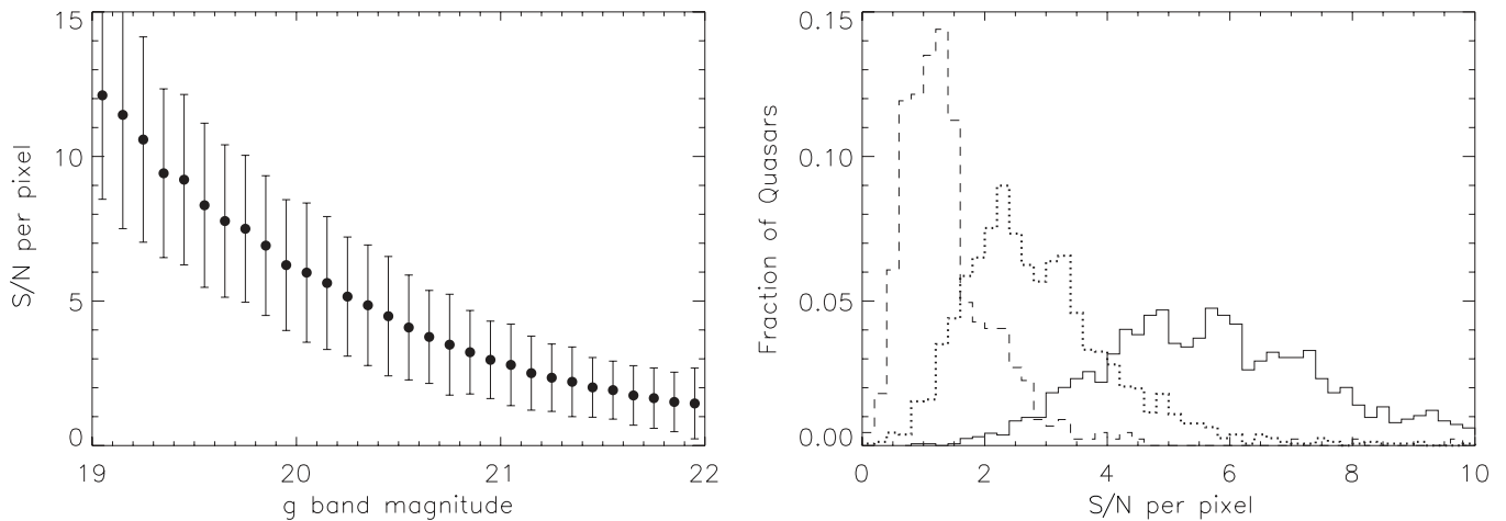
Figure 13. Statistics of the depth of the spectra in the Ly \alpha forest region 1041 Å to 1185 Å (rest frame). Only quasars at z > 2.5 are included, so that the entire Ly \alpha forest lies within BOSS wavelength coverage. On average, the sampling is bit more than 1 \text{ \AA pixel}^{-1} in this subsample. Left: mean S/N per pixel as a function of extinction-corrected g_{\text{PSF}} magnitude. The error bars represent the standard deviation of all quasars in each bin of width 0.1 mag. Right: distribution of the S/N per pixel. The solid line is taken from a sample of quasars near the bright end ( g_{\text{PSF}} \sim 20 ) of the sample. The dotted line represents a typical quasar ( g_{\text{PSF}} \sim 21 ). The dashed line shows quasars near the faint magnitude limit g_{\text{PSF}} \sim 22.0 of the CORE and BONUS target selection algorithms.
