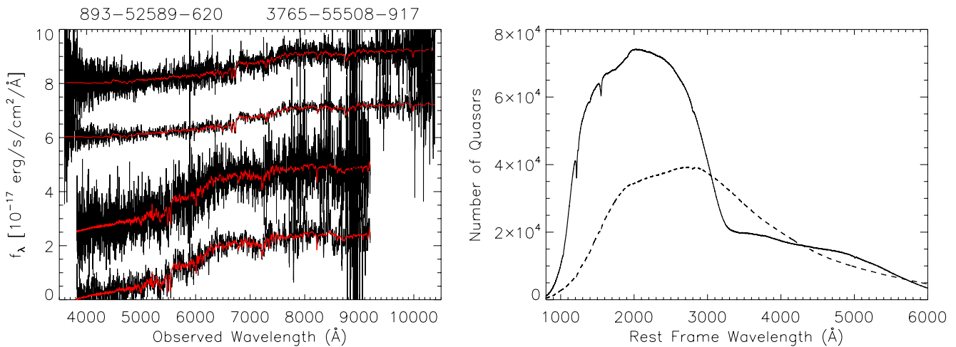
Figure 16. Left: comparison of the BOSS spectrum of one of the faintest CMASS targets ( z = 0.694 , i_{\text{fib}2} = 21.42 , \text{mean}(S/N/\text{pixel}) = 1.82 ) to the SDSS spectrum of one of the faintest LRG targets ( z = 0.395 , i_{\text{fib}} = 19.94 , corresponding to 3'' fiber, \text{mean}(S/N/\text{pixel}) = 2.38 ). From top to bottom, with offsets of 8, 6, 2, and 0 \times 10^{-17} \text{ erg s}^{-1} \text{ cm}^{-2} \text{ \AA}^{-1} , respectively, are the raw BOSS spectrum, the BOSS spectrum smoothed with a five pixel boxcar median filter, the raw SDSS spectrum, and the SDSS spectrum smoothed with a five pixel boxcar median filter. In all cases, the red curve represents the best-fit spectral template used to determine the redshift. The plate, MJD, and fiber combination for the two objects are displayed at the top of the panel. Right: corresponding spectral coverage of the quasar sample in BOSS (solid curve) relative to SDSS (dashed curve). The histogram represents the number of objects sampled at each rest-frame wavelength.
