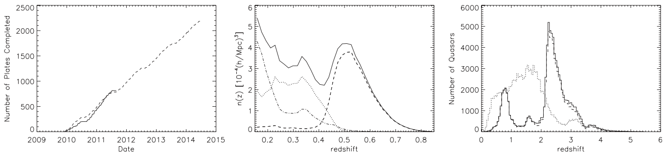
Figure 14. Left: progress of the survey at the time of DR9. The solid curve represents the number of unique plates completed as a function of time in the first two years of BOSS. The dashed curve represents the projected rate required to complete the baseline survey of 2208 plates. The yearly “pauses” are the result of the summer shutdown for telescope maintenance during the New Mexico monsoon season. The plate completion thresholds were changed in the summer of 2010 from S/N_R^2 = 26 to S/N_R^2 = 22 and from S/N_B^2 = 16 to S/N_B^2 = 10 . Center: average number density as a function of redshift for the SDSS (dash-dotted), LOWZ (dotted), and CMASS DR9 galaxies with ZWARNING_NOQSO = 0. Right: redshift distribution of DR7 (dotted), DR9 (solid), and unique DR9 (dashed) quasars.
