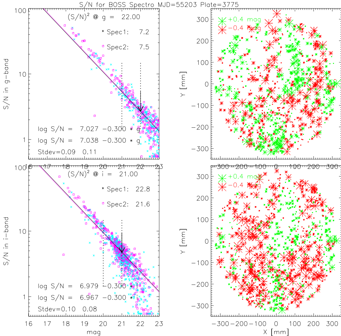
Figure 3. Example of the diagnostic from a series of four science exposures of plate 3775 that are produced in the quick reductions of data at APO. Similar plots become available to the observers less than five minutes after the end of an exposure. Left: cumulative signal-to-noise ratio (S/N in the figure captions) as a function of g_{\text{fib}2} (top) and i_{\text{fib}2} (bottom). Fibers from the two spectrographs are indicated by the blue symbol “x” (spectrograph 1) and a magenta square (spectrograph 2). The intercept of the linear fit of \log(S/N) as a function of magnitude and rms of that fit are computed for each spectrograph separately. Only fibers with fiber2 magnitudes in the range 21–22 (20–21) for the blue (red) cameras are used in the fit as indicated by the vertical dotted lines. The slope is held fixed at -0.3 as empirically determined from fits to the larger sample. This magnitude range is near the region of sky-limited noise and near the faint end of the main galaxy and quasar samples for the red and blue cameras, respectively. Right: the spatial profile of S/N over the plate. Red symbols represent fibers that fall below the best fit of the S/N linear solution that is represented by the solid line in the left-hand panels. Green symbols represent fibers that fall above the best linear fit of the S/N solution. The size of the symbol relates to the amount by which the fiber deviates, growing larger for fibers with larger deviation from the best fit. Guiding problems or other systematics can appear as coherent structure in this diagram. The distribution of objects that fall below the best-fit line is fairly uniform, indicating a lack of such effects for this particular plate. (A color version of this figure is available in the online journal.)
