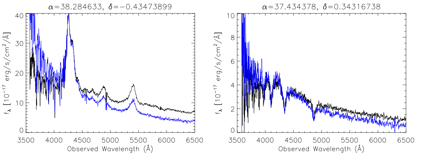
Figure 9. Quasar target spectra smoothed with a five-pixel median boxcar filter, covering the wavelength range 3500 Å through 6500 Å taken at different airmass, demonstrating the effects of atmospheric differential refraction and other guiding errors on spectrophotometry. Left: spectrum of a g_{\text{fib2}} = 19.48 quasar at z = 2.49 observed at an airmass of 1.2 (black) and again at an airmass of 1.4 (blue). Right: spectrum of a white dwarf with g_{\text{fib2}} = 21.53 on the same observations with the same color pattern.
