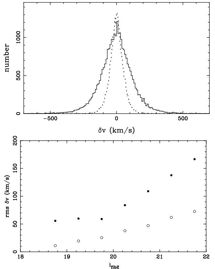
Figure 10. Statistics of \delta v in pairs of spectra for the same galaxy. Top: histogram of \delta v for RUNZ (solid black) and for idlspec2d (dashed). Bottom: rms width of distribution binned at half magnitude intervals in i_{\text{fib2}} . RUNZ is presented as solid circles while idlspec2d is presented as open circles.
