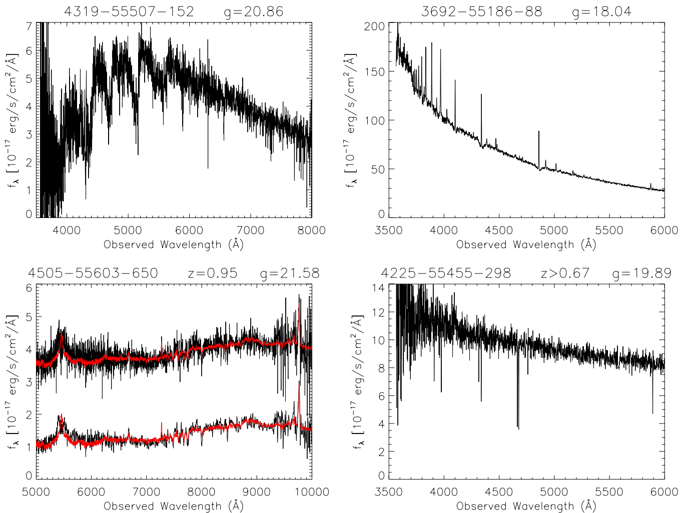
Figure 7. Mosaic of example spectra of rare objects discovered in the BOSS spectroscopic sample. Top: spectrum of a carbon star (left) and a cataclysmic variable with strong emission lines (right). Bottom: spectrum of a post-starburst galaxy at z = 0.95 with AGN activity (left) and a featureless BL Lac object imprinted with absorption lines from Fe II \lambda 2382 , Fe II \lambda 2600 , and the Mg II \lambda 2798, 2803 doublet at z = 0.67 (right). The idlspec2d template (red) for the post-starburst galaxy is a good fit to the data. For this galaxy, the raw data are displayed with an offset of 2.5 \times 10^{-17} \text{ erg s}^{-1} \text{ cm}^{-2} \text{ \AA}^{-1} and the spectrum smoothed with a five-pixel median boxcar filter is shown at true flux density.
