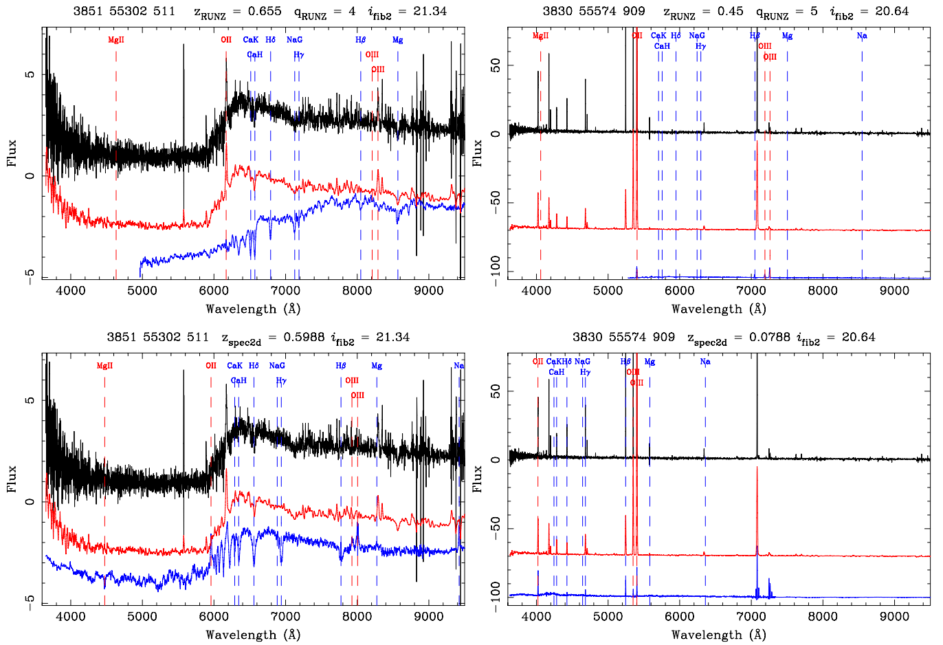
Figure 12. Examples of spectra that produced discrepant redshifts between the RUNZ analysis and the idlspec2d analysis where one is incorrect. The labels are the same as those in the previous figure. Left: example spectrum where manual classification reveals the RUNZ redshift to be correct and the idlspec2d redshift to be incorrect. The spectral distortion around 6000 Å is likely due to poor calibration in the dichroic region, a rare occurrence in BOSS spectra. Right: example spectrum where manual classification reveals the idlspec2d redshift to be correct and the RUNZ redshift to be incorrect.
