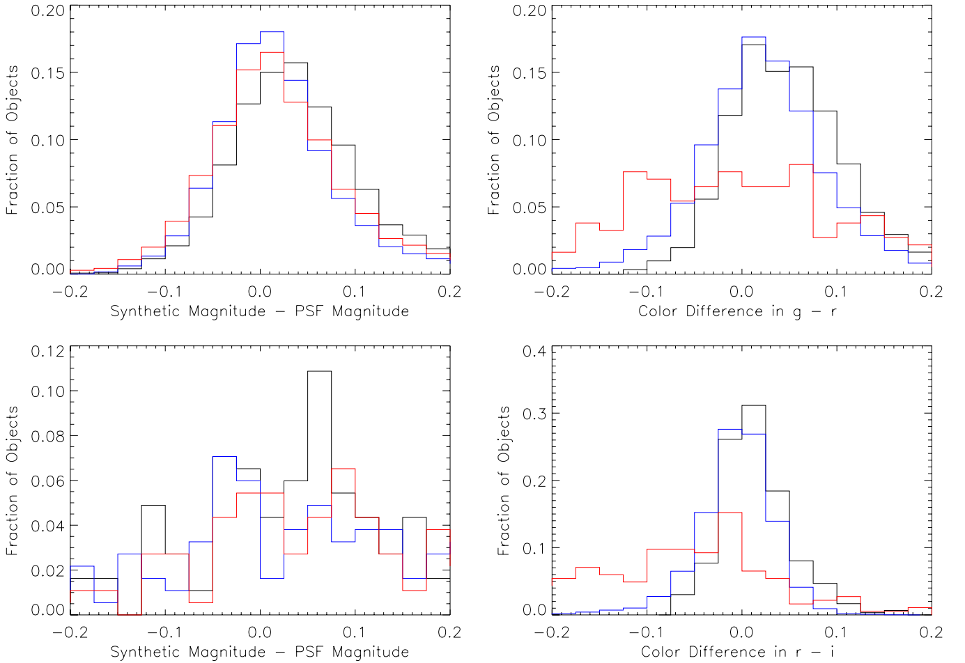
Figure 8. Difference between the synthetic photometry computed from each spectrum and the measured photometry from the SDSS imaging data. Left: histogram of the spectrophotometric offsets for stars. The black line shows g_{\text{synthetic}} - g_{\text{PSF}} for the standard stars (top) and for a sample of stars that appeared as contaminants in the CORE and BONUS quasar samples (bottom). Similarly, the blue lines show the offsets for the r filter while the red lines show the offsets for the i filter. Right: histogram of the color differences (g - r)_{\text{synthetic}} - (g - r)_{\text{PSF}} shown in the top panel and r - i in the bottom panel. Standard stars are presented as the blue line using PSF magnitudes, galaxies as the black line (fiber2 magnitudes), and stellar contaminants in the quasar sample as the red line (PSF magnitudes).
