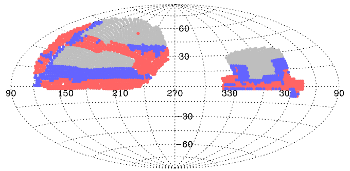
Figure 1. Location of pointing centers for the 2208 spectroscopic plates in the BOSS survey footprint in an Aitoff projection in J2000 equatorial coordinates. Gray circles represent the location of plates that remained to be drilled after the summer of 2011. Blue circles represent plates that were drilled and were ready to observe in the third year of the survey. Red circles represent the plates that were completed in either the first or second year of the survey, whose observations are released in DR9.
