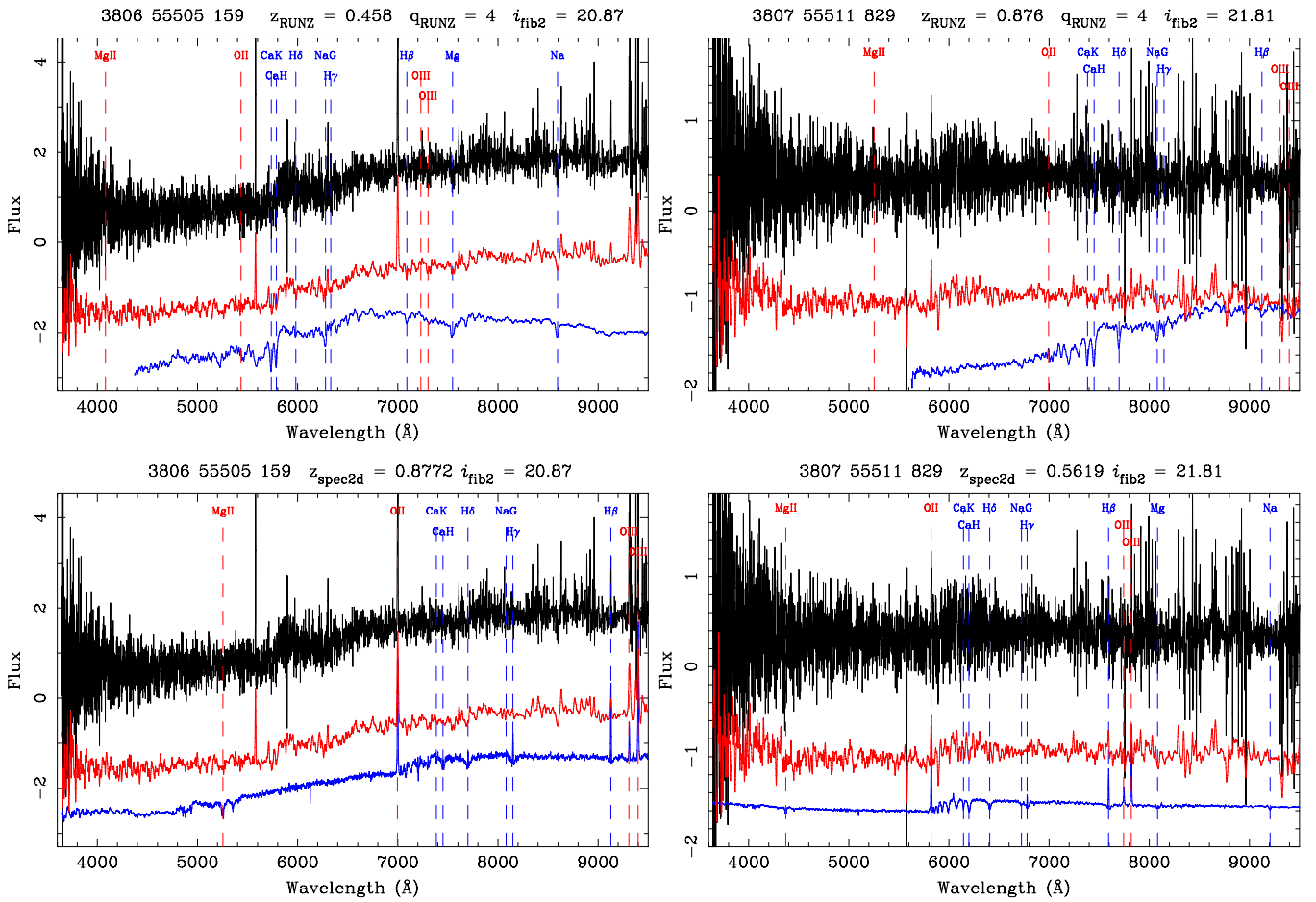
Figure 11. Examples of spectra that produced discrepant redshifts between the RUNZ analysis and the idlspec2d analysis due to a superposition of multiple objects. The RUNZ fit is shown in the top panels and the idlspec2d fit in the bottom panels. Three spectra are plotted in each panel, from top to bottom: raw BOSS spectrum, BOSS spectrum smoothed with a 7 pixel boxcar filter, and best-fit spectral template. Typical line features are identified at the top of each panel by name, flux density is presented in arbitrary units. As before, the plate, MJD, fiber combination is presented at the top of each panel. Left: example spectrum where the RUNZ redshift corresponds to a foreground passive galaxy and the idlspec2d redshift corresponds to a background emission-line galaxy. Right: example spectrum where the RUNZ redshift corresponds to a background passive galaxy and the idlspec2d redshift corresponds to a foreground emission-line galaxy.
