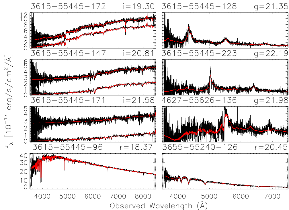
Figure 6. Mosaic of BOSS spectra (black) and best-fit idlspec2d templates (red) of varying luminosity. The plate, MJD, fiber, and fiber2 magnitude are listed at the top of each panel. Left (top three panels): Galaxy spectra from the LOWZ and CMASS samples in order of decreasing luminosity and increasing redshift: a z = 0.238 LOWZ galaxy, a z = 0.541 CMASS galaxy, and a z = 0.695 CMASS galaxy that is slightly fainter than the i_{\text{fib2}} < 21.5 threshold that was imposed after year one. In each case, the top spectrum is offset by 2.5 \times 10^{-17} \text{ erg s}^{-1} \text{ cm}^{-2} \text{ \AA}^{-1} and the bottom spectrum is smoothed with a five-pixel median boxcar filter. Right (top three panels): unsmoothed quasar spectra from the CORE and BONUS samples in order of increasing redshift: a z = 2.57 quasar, a z = 3.14 quasar, and a z = 3.53 quasar. Bottom: unsmoothed spectrum of a standard star (left) and of a white dwarf star (right).
