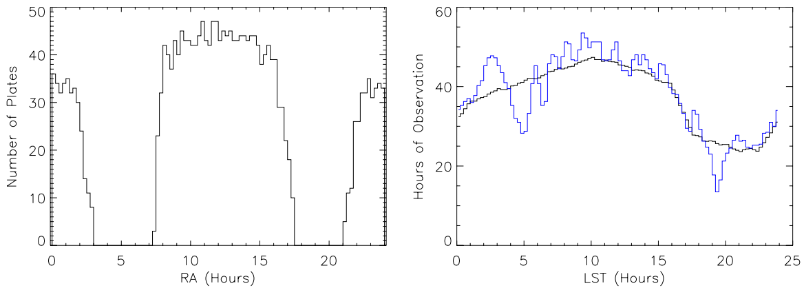
Figure 4. Left: distribution of plates in the BOSS footprint binned in 15 minute increments in right ascension. Right: number of hours of observing time available as a function of LST (black line) and the simulated time required at each LST to observe the full survey (blue line). The observing time is sampled in 15 minute increments and assumes a uniformly distributed 45% efficiency after weather loss. The discrete sum of the entries under the black line is equal to 3585 hr. The final simulated LST distribution shown in blue is discussed in Section 5.5.
