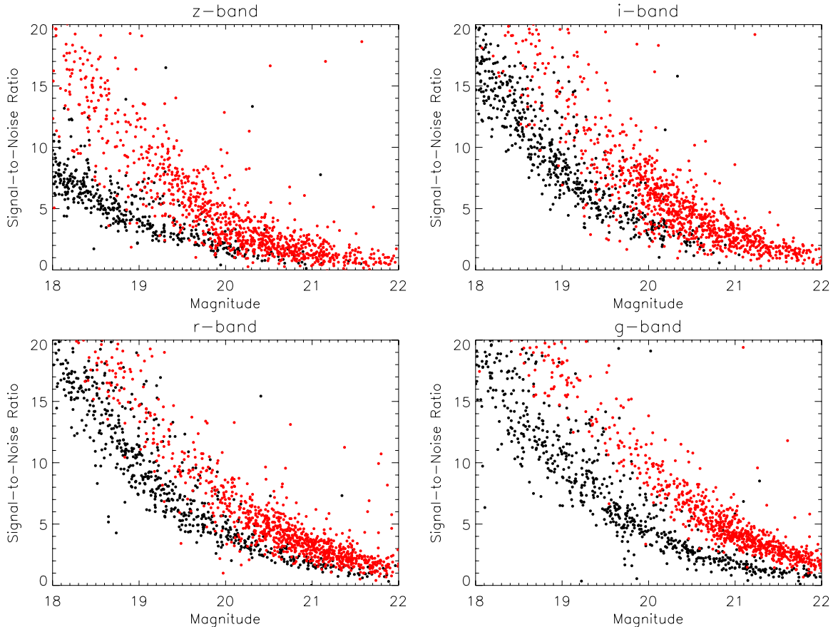
Figure 15. S/N per pixel as a function of extinction-corrected PSF magnitude in each of the four synthetic bandpass filters ( griz ) matching the photometric passbands of the SDSS imaging survey. In each case, the red dots represent BOSS data while the black dots represent SDSS data. The data were selected from a random sampling of objects classified as stars over the full SDSS and BOSS samples.
