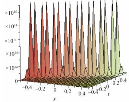
Figure 7. Solitons solution for \lambda = 4, \mu = 4, \alpha = 1.5, \beta = 5 \times 10^{-11}, U = 0.75, V = 24 .
