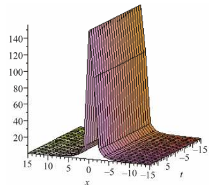
Figure 9. Periodic solution for \lambda = 8, \mu = 16, \alpha = 5 \times 10^{-6}, \beta = 0.125, U = 5, V = 9 .
