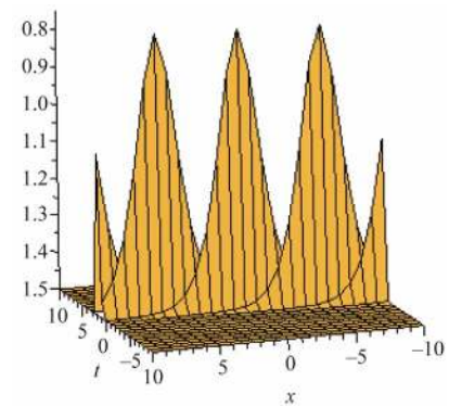
Figure 5. Solitons solution for \lambda = 3, \mu = 2, \alpha = 7, \beta = 2 .
