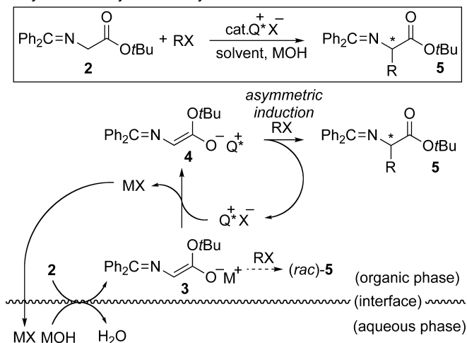
Scheme 1.5
