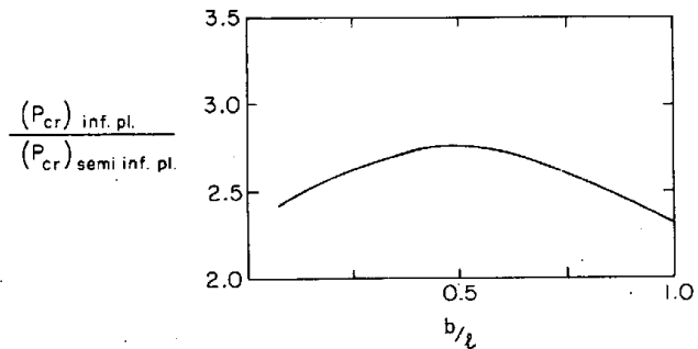
Figure 8. (P_{cr})_{inf pl} / (P_{cr})_{semi inf pl} vs b/l .
