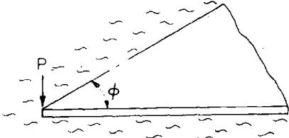
Figure 11. Floating wedge shaped plate of opening angle \phi subjected to load P at the tip.
