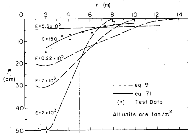
Figure 24. Comparison of ice plate deflections due to loads of short duration at 0^{\circ}\text{C} . 131
