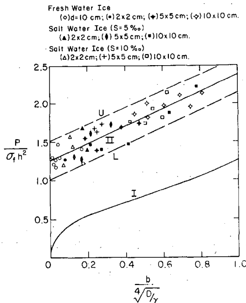
Figure 25. Laboratory test results for infinite plates. 98
