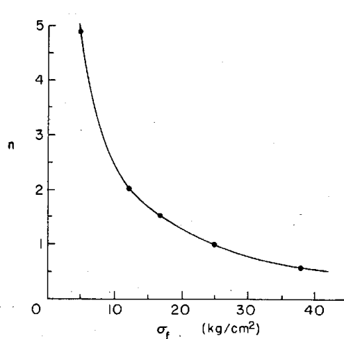
Figure 1. Correction coefficient n as related to failure stress \sigma_f (Korunov 70 ).
