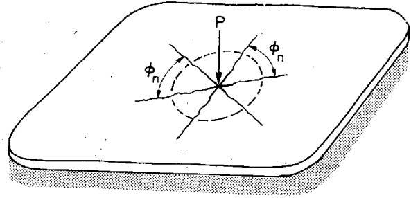
Figure 13. Failure mechanism for a large floating plate subjected to a load P .
