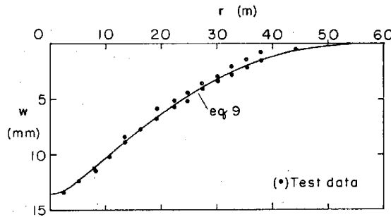
Figure 23. Comparison of ice plate deflections due to loads of short duration at -15^{\circ}\text{C} < T < -7^{\circ}\text{C} .
