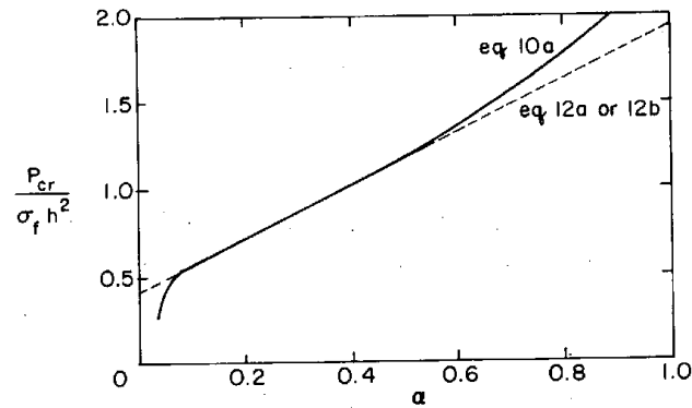
Figure 4. P_{cr}/\sigma_f h^2 vs \alpha .
