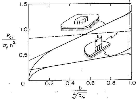
Figure 7. Comparison of analytical results. 98
