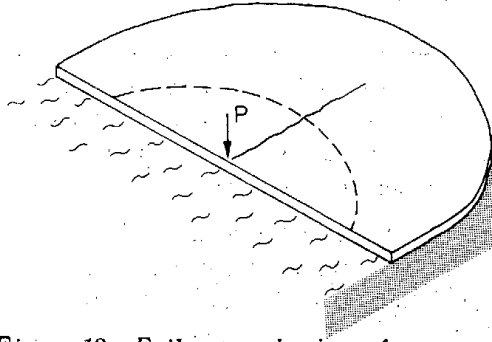
Figure 12. Failure mechanism of a floating semi-infinite plate subjected along the free edge to a load P .
