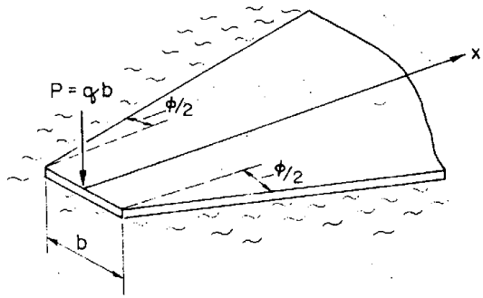
Figure 14. Wedge shaped plate subjected to a load P = qb .
