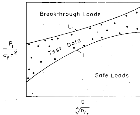
Figure 26. Illustration of new concept for evaluating breakthrough loads from test data.
