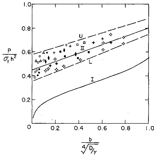
Figure 27. Results for semi-infinite plate. 98 (Symbols as in Fig. 25.)
