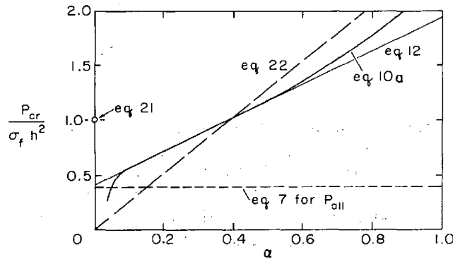
Figure 5. A comparison of approximations for P_{cr} with exact graph.
