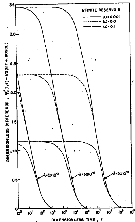
FIG. 6 — DEVIATION FROM THE ASYMPTOTE.
