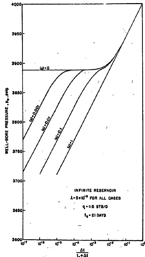
FIG. 8 — THEORETICAL BUILD-UP CURVES.
