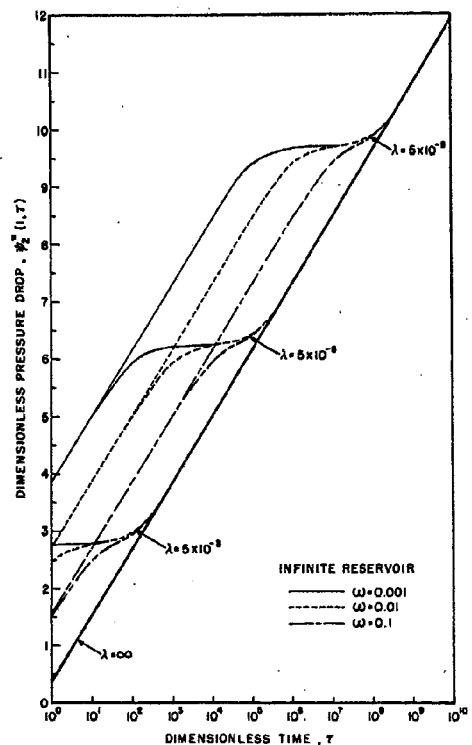
FIG. 5 — SOLUTIONS OBTAINED BY APPROXIMATE INVERSION.
