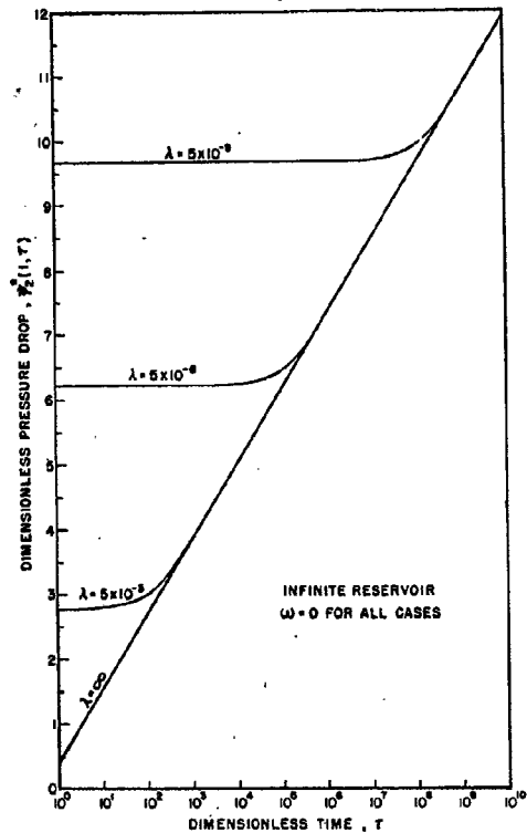
FIG. 3 — SOLUTIONS OBTAINED BY APPROXIMATE INVERSION.
