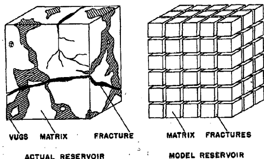
FIG. 1 — IDEALIZATION OF THE HETEROGENEOUS POROUS MEDIUM.
