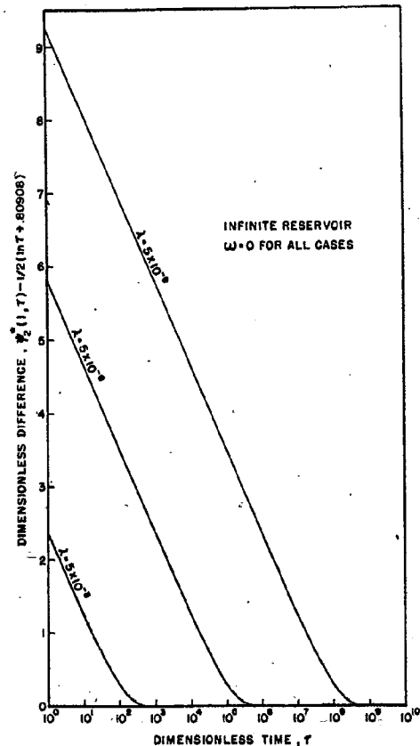
FIG. 4 — DEVIATION FROM THE ASYMPTOTE.
