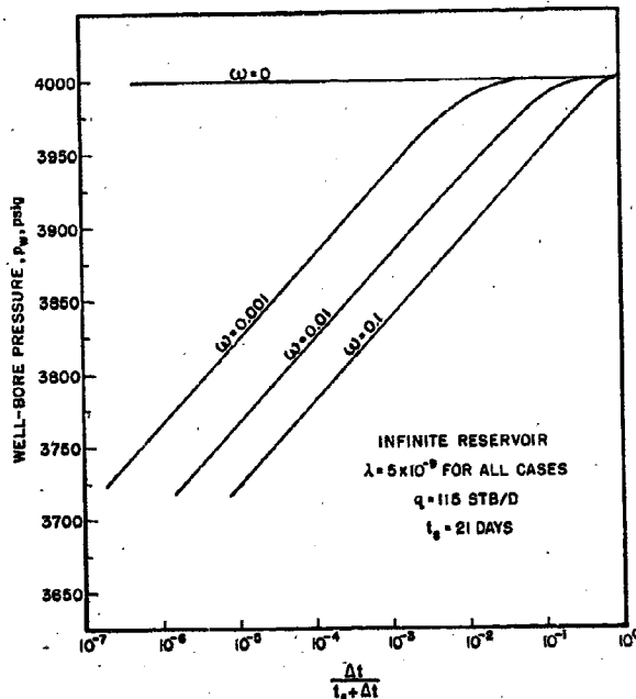
FIG. 7 — THEORETICAL BUILD-UP CURVES.
