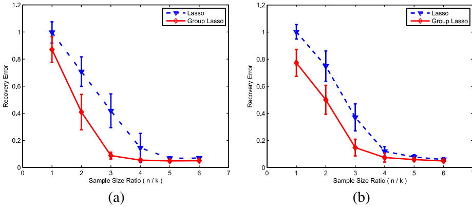
FIG. 5. Recovery performance: (a) g active groups have randomly uneven group sizes; (b) half of g active groups are single element groups and another half of g active groups have large group size.
