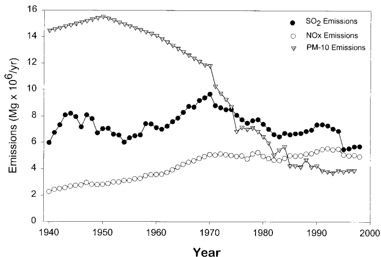
Figure 4. Long-term trends in emissions of \text{SO}_2 (●), and \text{NO}_x (○) for the HBEF source area and particulate matter 10 \mu\text{m} in size (PM-10; ▼), excluding fugitive dust sources for the U.S. (US EPA 2000). The pattern of PM-10 emissions for the smaller HBEF source region would follow the same general trends as for the US source area assuming that sources and air-mass trajectories were similar to the relationships found for \text{SO}_2 and \text{NO}_x emissions on a regional and national level.
