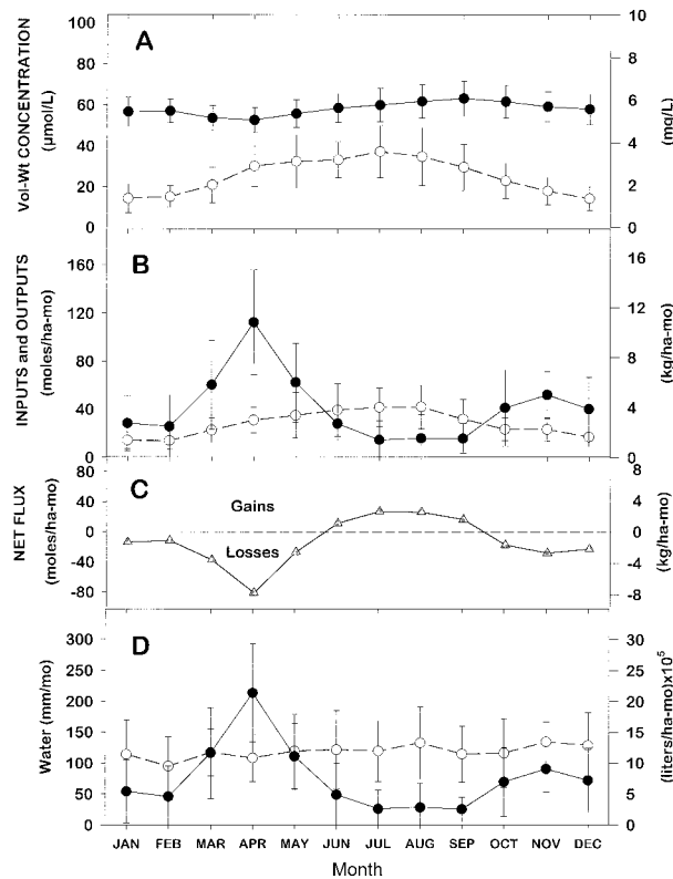
Figure 6. A. Average monthly volume-weighted concentrations of \text{SO}_4^{2-} in bulk deposition ( \circ ) and stream water ( \bullet ) for W6 at HBEF during 1964–1998. The vertical bars are \pm one standard deviation for the mean value. B. Average monthly inputs of \text{SO}_4^{2-} in bulk deposition ( \circ ) and outputs of \text{SO}_4^{2-} in stream water ( \bullet ) for W6 during 1964–1998. The vertical bars are \pm one standard deviation for the mean value. C. Average monthly net flux of \text{SO}_4^{2-} (average bulk deposition input minus average stream-water output from B above) for W6 during 1964–1998. D. Average monthly amounts of precipitation ( \circ ) and stream water ( \bullet ) for W6 during 1964–1998. The vertical bars represent \pm one standard deviation for the mean value.
