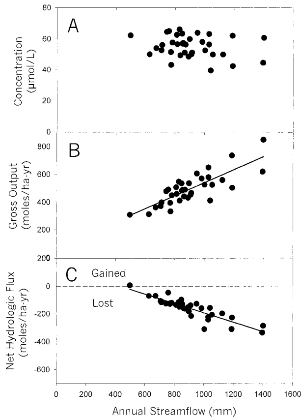
Figure 19. Relationship between the: A. Annual volume-weighted concentration of \text{SO}_4^{2-} in stream water and amount of annual streamflow. B. Annual gross output of \text{SO}_4^{2-} in stream water and amount of annual streamflow. The probability for a larger F-ratio for the regression line for 1964–1997 is p < 0.001 ; r^2 = 0.70 , and C. Net hydrologic flux for \text{SO}_4^{2-} (streamwater output minus bulk deposition input) for W6 at HBEF during 1964–1998. Negative fluxes indicate that the watershed-ecosystem lost \text{SO}_4^{2-} .
