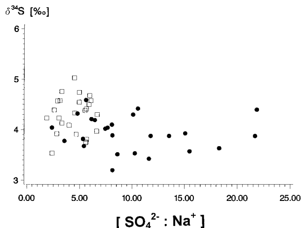
Figure 10. \delta^{34}\text{S} values (‰) related to the [\text{SO}_4^{2-} : \text{Na}^+] ratio in bulk deposition at W6 of the HBEF. \square = winter; \bullet = summer (modified from Alewell et al. (2000)).
