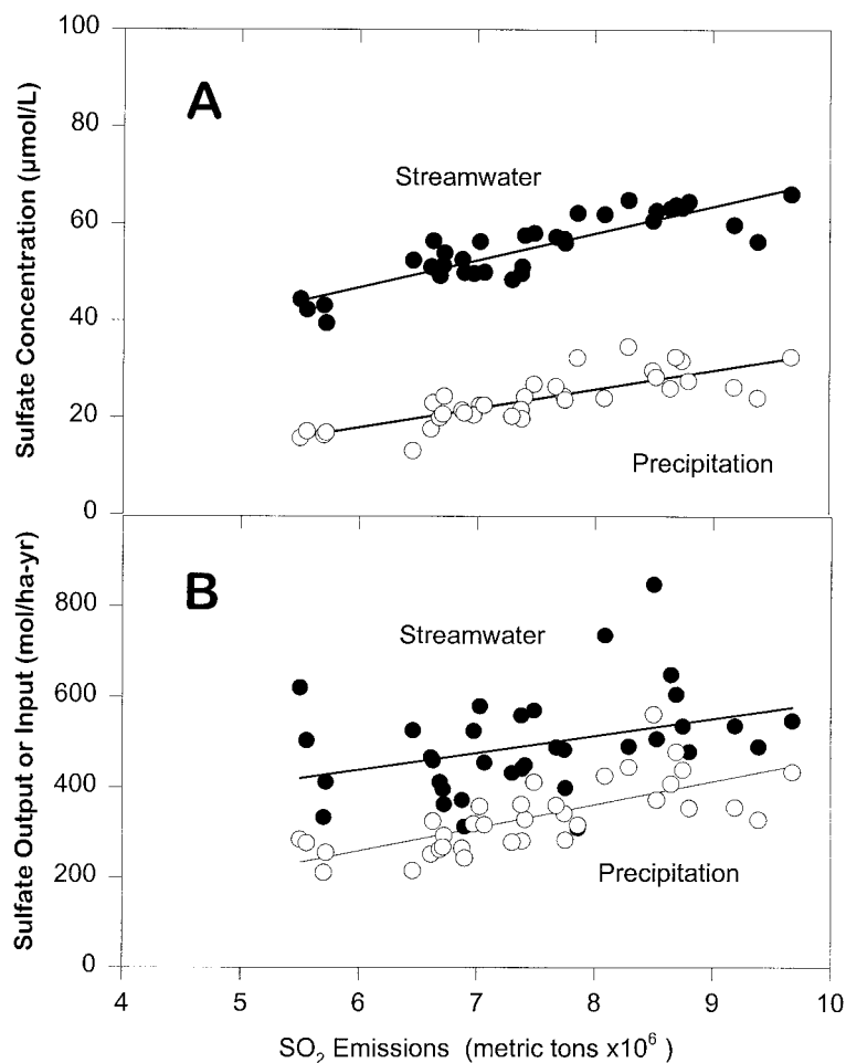
Figure 5. Relation between: A. sulfate concentrations in bulk deposition (-○-) or stream water (-●-) for the HBEF and SO 2 emissions for source region based on 15-hr air-mass, back trajectories (Butler et al. 2001; Likens et al. 2001) during 1970–1997. ( r^2 for bulk deposition is 0.65, and for stream water is 0.75). B. sulfate inputs in bulk deposition or outputs in stream water and SO 2 emissions for the HBEF source region during 1970–1997 ( r^2 for inputs is 0.51, and for outputs is 0.13).
