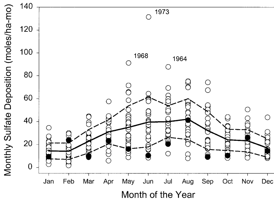
Figure 26. Atmospheric \text{SO}_4^{2-} input: individual monthly bulk deposition values during 1964–1998 (○); many values overlap; average monthly deposition (—) \pm SD (- -) during the 36 months of 1964–1998, and monthly deposition values during the 1983–1984 water-year (●).
