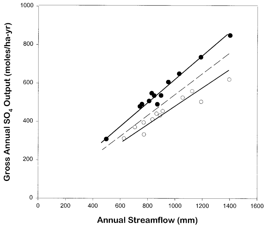
Figure 21. Changing relationship between the gross, annual output of \text{SO}_4^{2-} in stream water and the amount of annual streamflow for W6 at HBEF during 1964–1998. Symbols: \bullet is 1964–1965 to 1974–1975 and \circ is 1986–1987 to 1997–1998; the dashed line is the regression for all data, 1964–1965 to 1997–1998.
