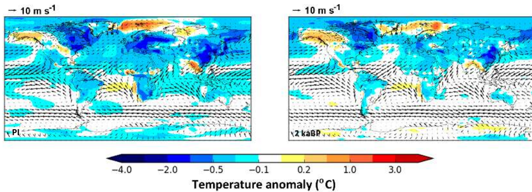
Figure 6. DJF surface temperature anomalies for KK10–control and KK10 surface winds for the late pre-industrial (1850 CE) and 2 ka BP.
