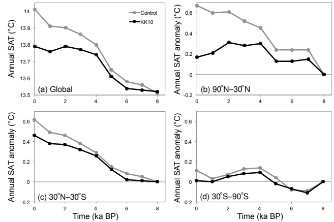
Figure 13. Time series plots for the Holocene simulations from HadCM3. Panel (a): annual mean global surface air temperature (SAT) for the control simulation in grey, and KK10 simulation in black; panel (b): anomaly in northern extratropical (30–90° N) annual mean temperature from the equivalent simulation at 8 ka BP; panel (c): same as (b) but for the tropics (30° N–30° S); panel (d): same as (b) but for the southern extratropics (30–90° S).
