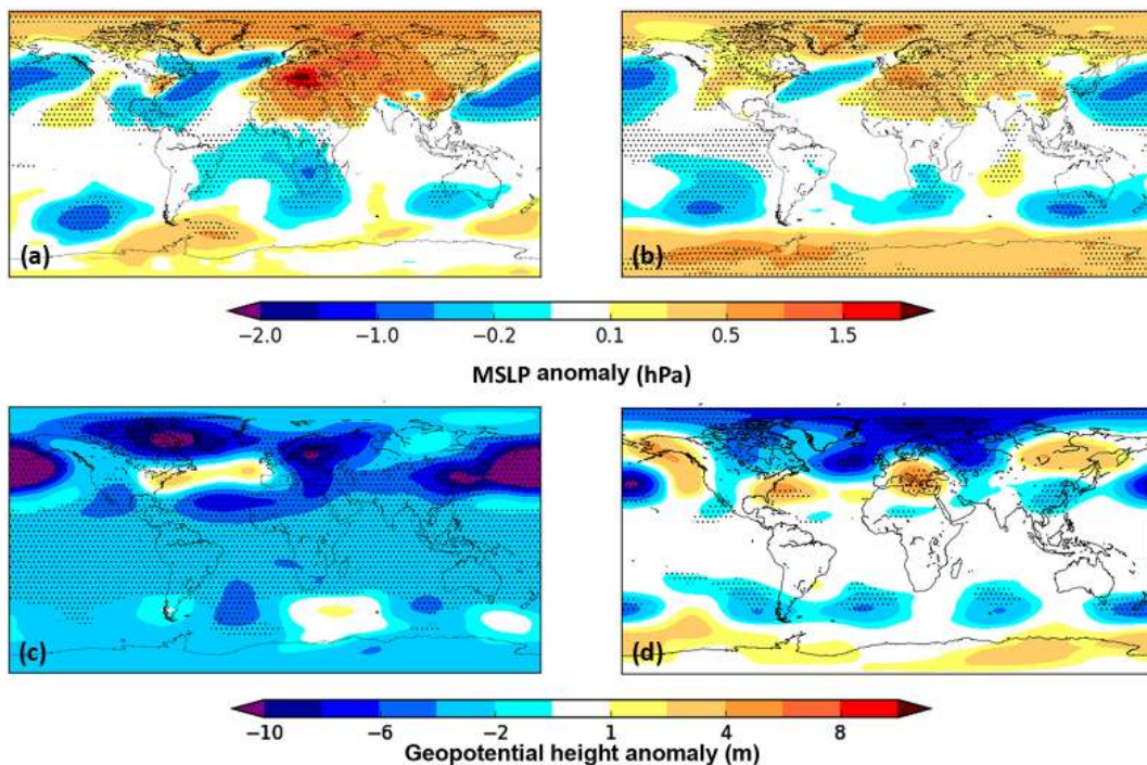
Figure 7. Modifiers of climate in regions outside the areas of anthropogenic land use change. All anomalies are for KK10–control: (a) JJA MSLP changes at 1850 CE, with the stippling indicating grid boxes where the anomalies are significant at the 95 % level using Wilcoxon rank sum statistical analysis; (b) as (a) but for 4 ka BP; (c) DJF 500Pa geopotential height anomalies at 1850 CE demonstrating stationary wave pattern, with the stippling indicating grid boxes where the anomalies are significant at the 95 % level using Wilcoxon rank sum statistical analysis; (d) as (c) but for 4 ka BP.
