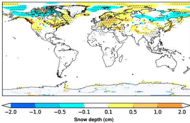
Figure 12. DJF snow depth anomalies (cm) for KK10 minus control for the late pre-industrial period (1850 CE). The stippling indicates grid boxes where the anomalies are significant at the 95 % level using Wilcoxon rank sum statistical analysis.
