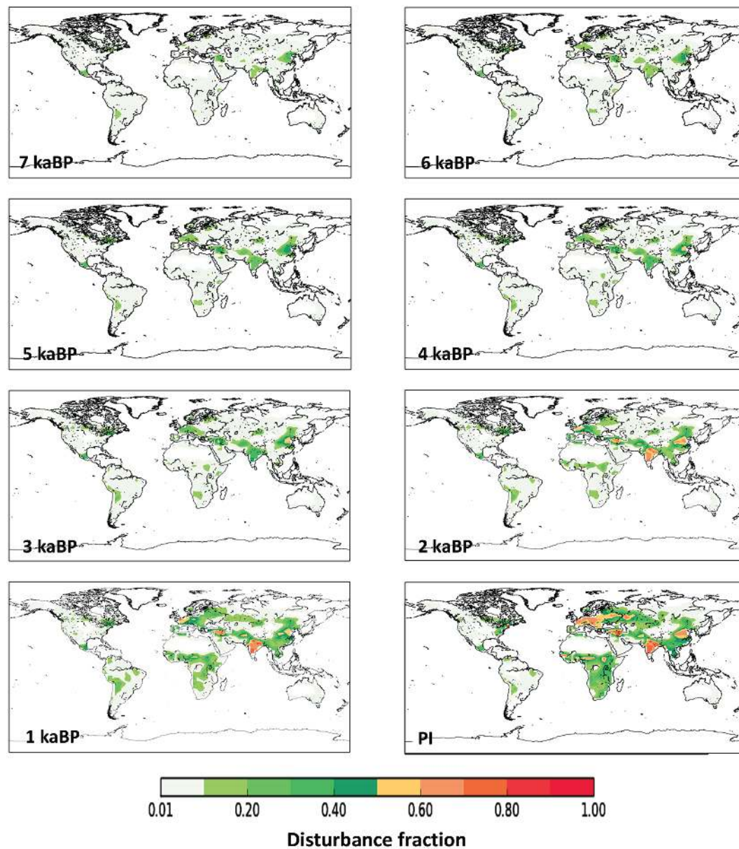
Figure 1. Fraction of anthropogenically disturbed land at 1000-year intervals from the late pre-industrial (1850 CE) period to 7 ka BP. The land disturbance data are based on the anthropogenic land use scenario KK10 (Kaplan et al., 2009, 2011).
