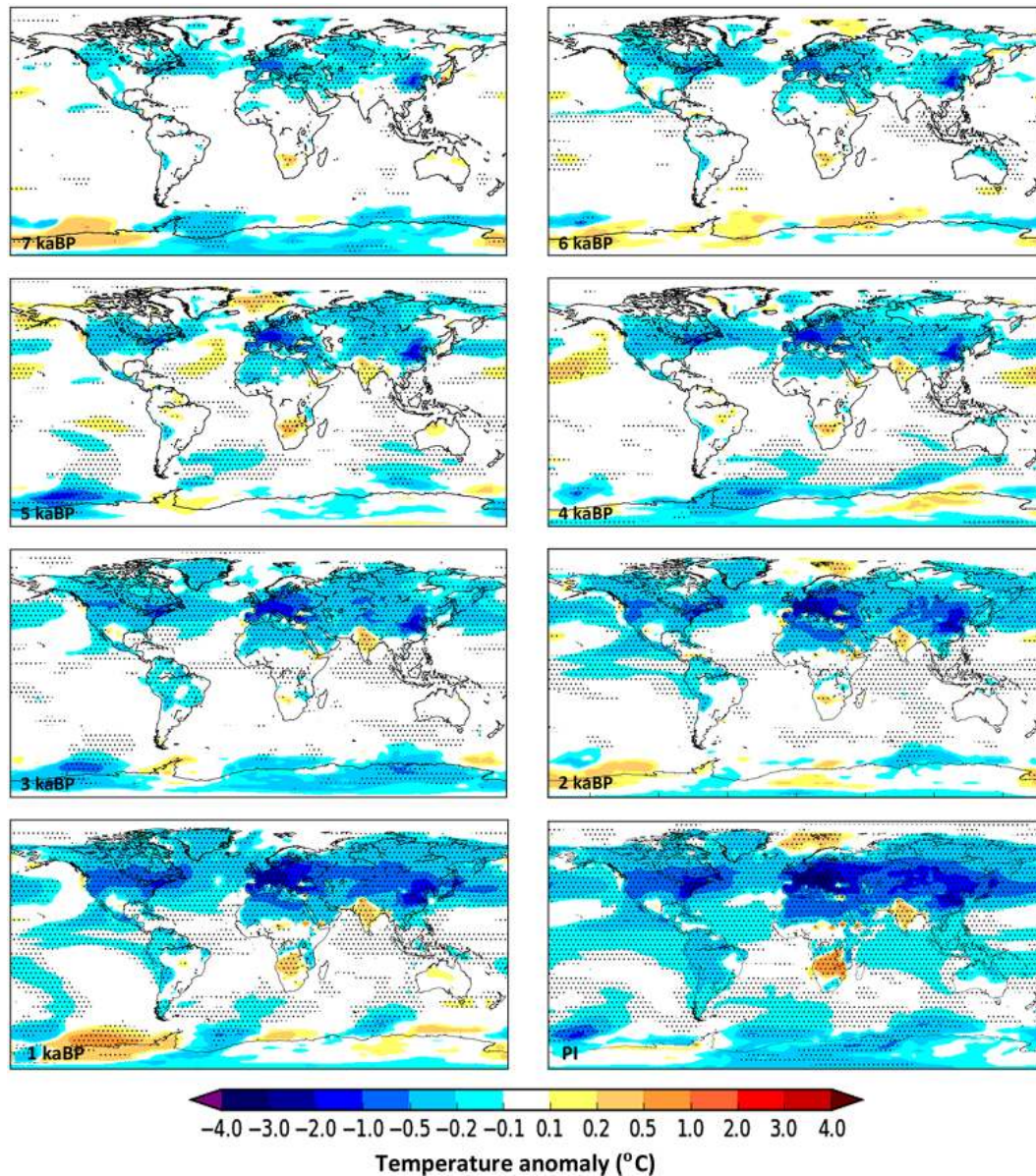
Figure 2. JJA temperature anomalies ( ^{\circ}\text{C} ) for KK10 minus control at time slices from the late pre-industrial period (1850 CE) to 7 ka BP. The stippling indicates grid boxes where the anomalies are significant at the 95 % level using Wilcoxon rank sum statistical analysis.
