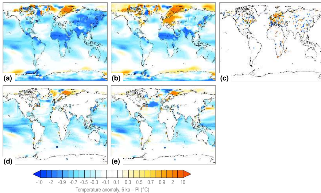
Figure 14. Mid-Holocene minus pre-industrial temperature anomalies: (a) annual mean surface air temperature anomalies from the control experiment; (b) annual mean surface air temperature anomalies from the KK10 experiment; (c) Bartlein et al. (2011) pollen-based reconstructions of the mean annual air temperature anomaly; (d) ocean annual mean temperature for the top two layers (25 m) from the control experiment with palaeo-proxy reconstructions (Marcott et al., 2013) overlaid in coloured circles; (e) as in (d) but for the KK10 experiment.
