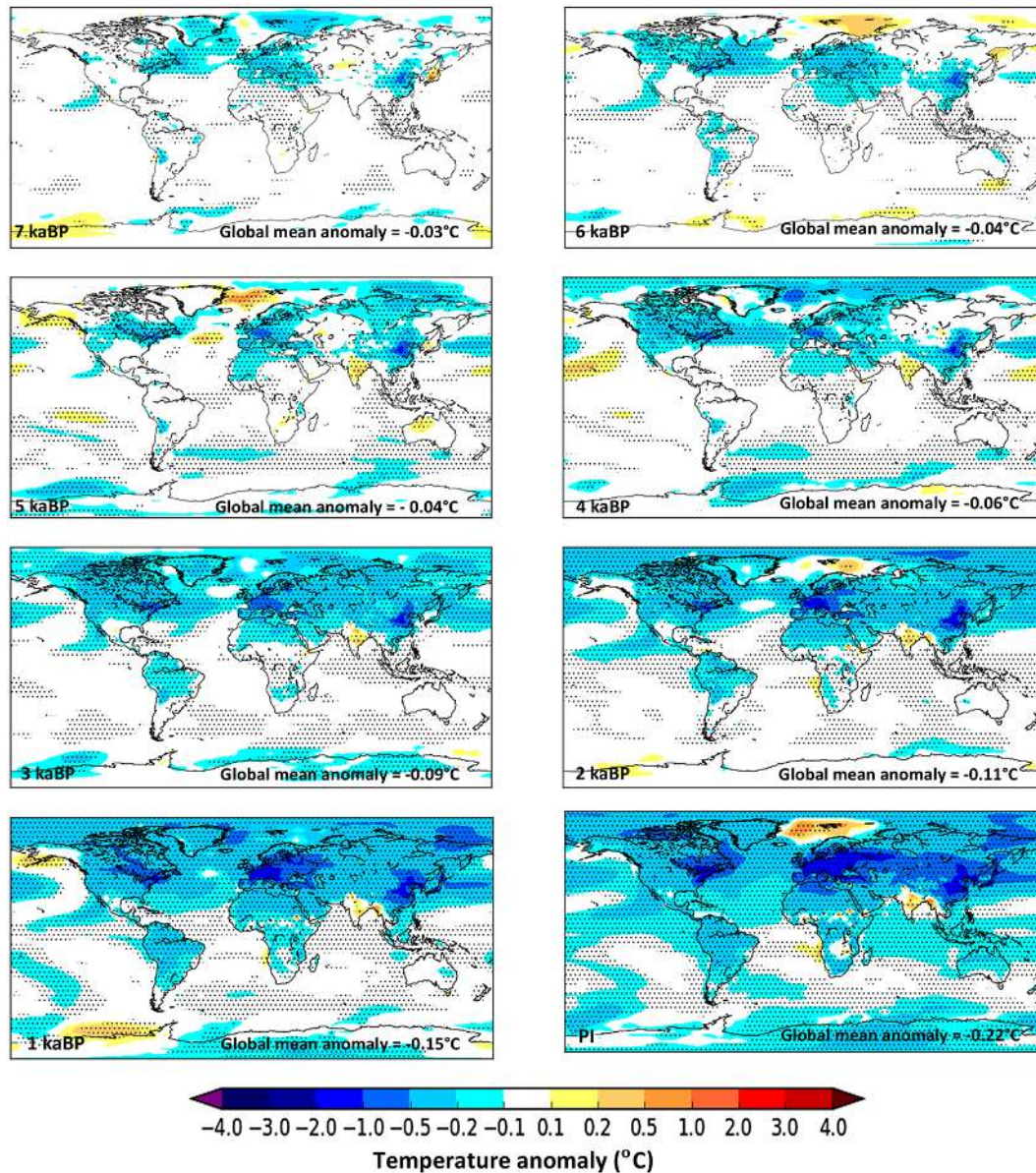
Figure 4. Annual temperature anomalies (°C) for KK10 minus control at time slices from the late pre-industrial period (1850 CE) to 7 ka BP. The stippling indicates grid boxes where the anomalies are significant at the 95 % level using Wilcoxon rank sum statistical analysis.
