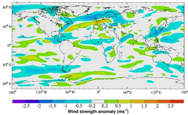
Figure 10. JJA 850 hPa wind strength anomalies ( \text{ms}^{-1} ) for KK10 minus control for the late pre-industrial period (1850).
