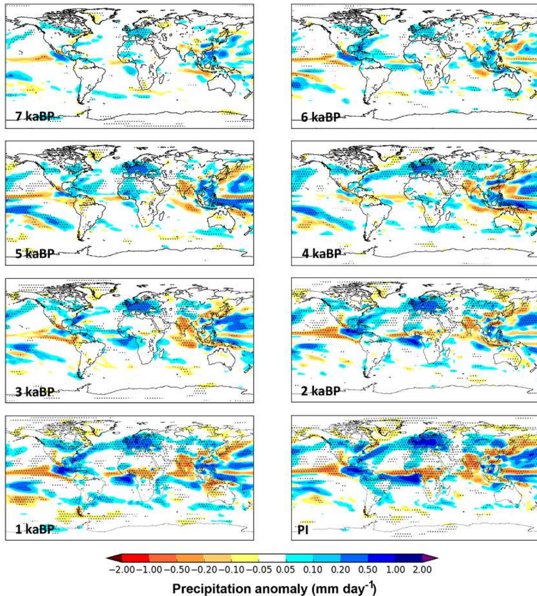
Figure 8. JJA precipitation anomalies ( \text{mm day}^{-1} ) for KK10 minus control at time slices from the late pre-industrial period (1850 CE) to 7 ka BP. The stippling indicates grid boxes where the anomalies are significant at the 95 % level using Wilcoxon rank sum statistical analysis.
