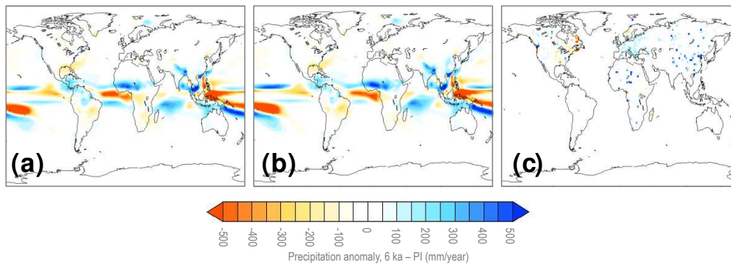
Figure 15. Mid-Holocene minus pre-industrial precipitation anomalies: (a) annual mean precipitation anomalies from the control experiment; (b) annual mean precipitation anomalies from the KK10 experiment; (c) Bartlein et al. (2011) pollen-based reconstructions of the mean annual precipitation anomaly.
