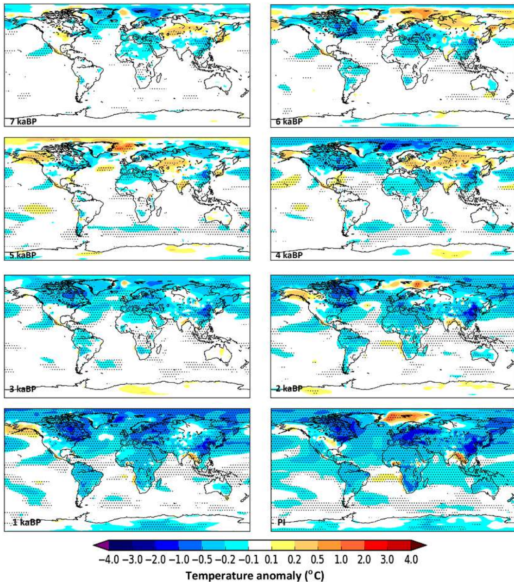
Figure 3. DJF temperature anomalies ( ^{\circ}\text{C} ) for KK10 minus control at time slices from the late pre-industrial period (1850 CE) to 7 ka BP. The stippling indicates grid boxes where the anomalies are significant at the 95 % level using Wilcoxon rank sum statistical analysis.
