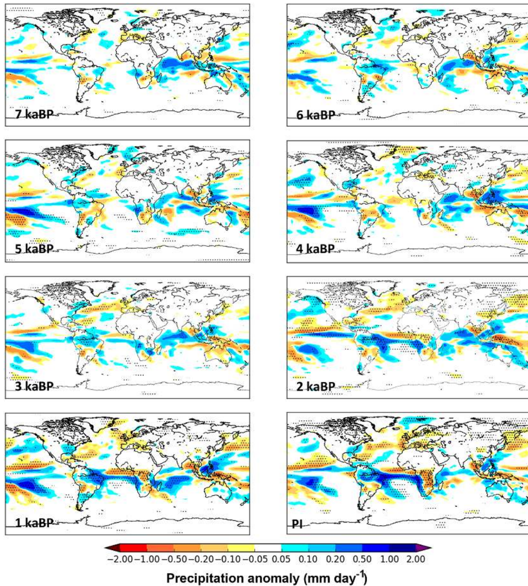
Figure 9. DJF precipitation anomalies ( \text{mm day}^{-1} ) for KK10 minus control at time slices from the late pre-industrial period (1850 CE) to 7 ka BP. The stippling indicates grid boxes where the anomalies are significant at the 95 % level using Wilcoxon rank sum statistical analysis.
