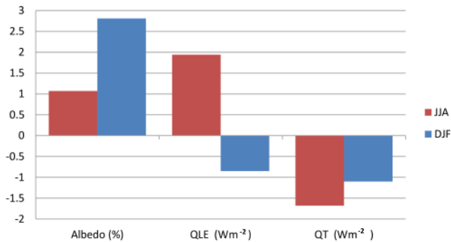
Figure 16. JJA and DJF albedo, latent heat flux (QLE), and turbulent heat flux (QT) anomalies for KK10 minus control for the late pre-industrial period (1850 CE) for the North America–Eurasia land surface.
