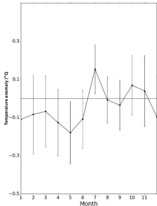
Figure 11. Indian temperature seasonality; KK10–control surface temperature anomalies for the late pre-industrial (1850 CE) simulation; the vertical bars indicate the normal range of variability which is considered to be within 2 standard deviations of the mean.
