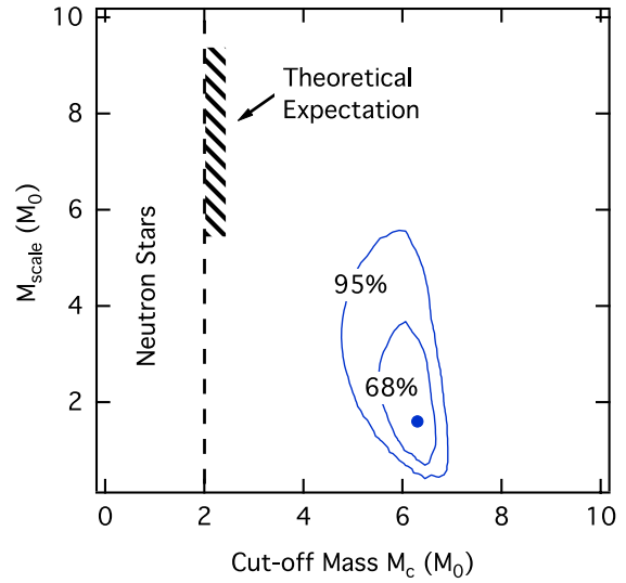
Figure 3. Parameters of an exponential black hole mass distribution with a low-mass cutoff. The cutoff mass is well above theoretical expectations, indicating a sizable gap between neutron-star and black hole masses. Furthermore, the mass scale in the exponential is significantly smaller than theoretical expectations. (A color version of this figure is available in the online journal.)
