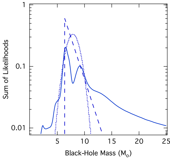
Figure 2. Solid line shows the sum of likelihoods for the mass measurements of the 16 black holes in low-mass X-ray binaries. Note that because of the high-mass wings of the individual likelihoods, the shape of their sum is artificial at the high-mass end. The dashed and dotted lines show the exponential and Gaussian distributions, respectively, with parameters that best fit the data (see Section 4). (A color version of this figure is available in the online journal.)
