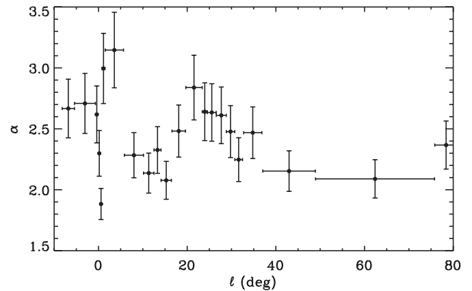
Figure 18. Power-law index on the flux density distribution as a function of Galactic longitude, derived for groups of 50 sources above the survey completeness limit of 0.4 \text{ Jy} . The flux densities are measured in 40'' apertures across the Galactic plane.
