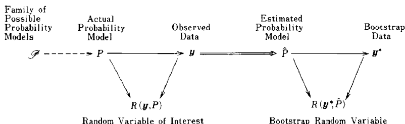
Fig. 8 A schematic illustration of the bootstrap process for a general probability model P . The expectation of R(\mathbf{y}, P) is estimated by the bootstrap expectation of P(\mathbf{y}^*, \hat{P}) . The double arrow indicates the crucial step in applying the bootstrap.
