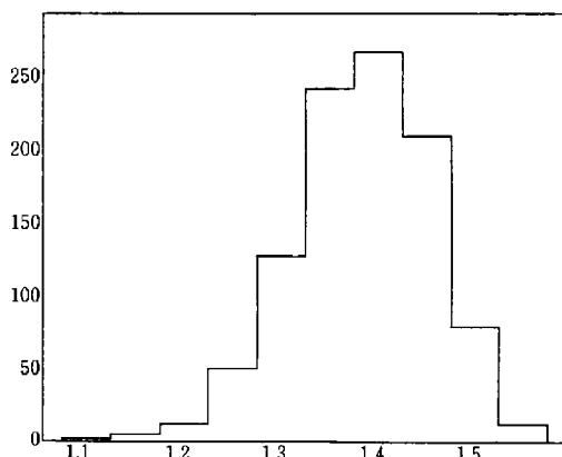
Fig. 11 Bootstrap histogram of \hat{a}_1^*, \dots, \hat{a}_{1000}^* for the Wolfer sunspot data, model (6.2).
