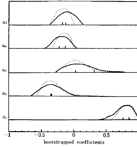
Fig. 4 Smoothed histograms of the bootstrapped coefficients for the first term in the projection pursuit regression model. Solid histograms are for the usual projection pursuit model; the dotted histograms are for linear \hat{s}(\cdot) .
