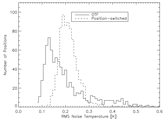
FIG. 9.—Comparison of the rms noise temperature, \sigma(T_A^*) , for OTF and position-switched data. For the comparison, we use a small region of the survey ( 40^\circ \leq l \leq 40^\circ.1 and -0^\circ.3 \leq b \leq 0^\circ ) that was observed in both of these modes. The improved sensitivity of the OTF data (peak at 0.13 K) compared to the position-switched data (peak at 0.20 K) is clearly evident. The data are binned by 0.01 K intervals.
