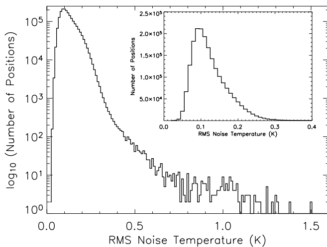
FIG. 8.—Histogram of the rms noise temperature, \sigma(T_A^*) , for all (l, b) positions in the GRS. The rms noise temperatures were determined using data from 130 to 135 \text{km s}^{-1} for l \leq 40^\circ and from 80 to 85 \text{km s}^{-1} for l > 40^\circ . The inset shows the same histogram but on a linear rather than logarithmic scale. The data are binned by 0.01 K intervals.
