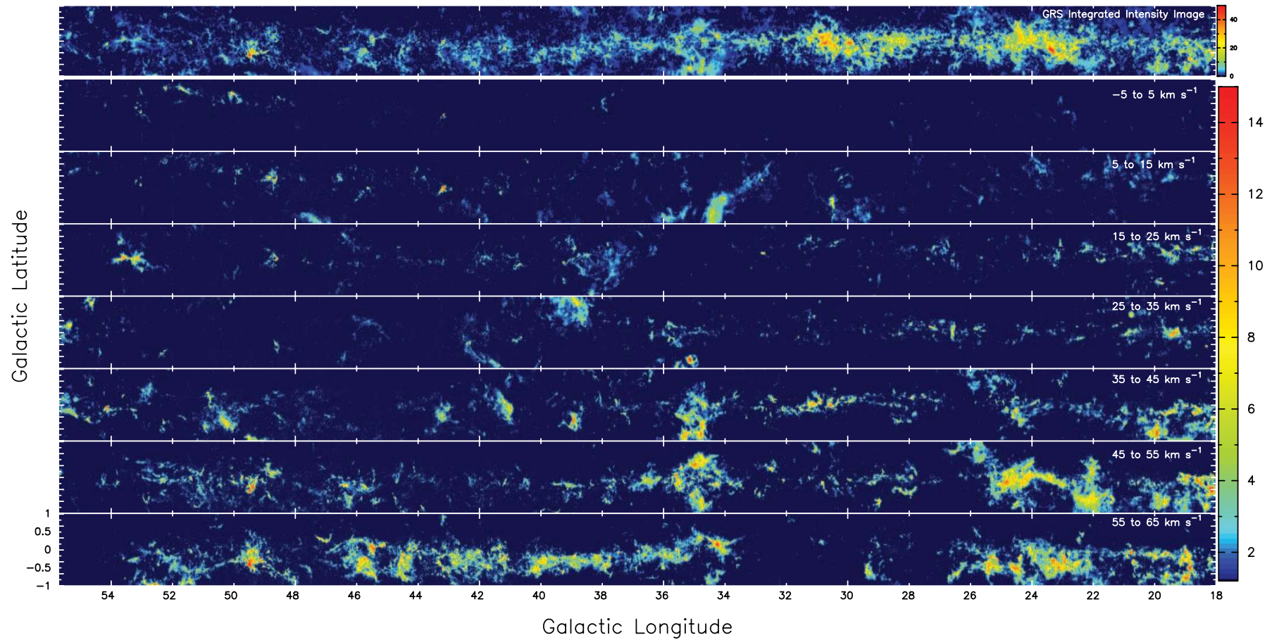
FIG. 2.—Channel maps of GRS ^{13}\text{CO} emission. The maps were made by integrating the emission over 10 \text{ km s}^{-1} velocity bins. The image units are in \text{K km s}^{-1} . The top image shows the integrated intensity image from Fig. 1 for comparison. The velocity range of each image is labeled. The channel maps clearly separate emission features along the same line of sight.
