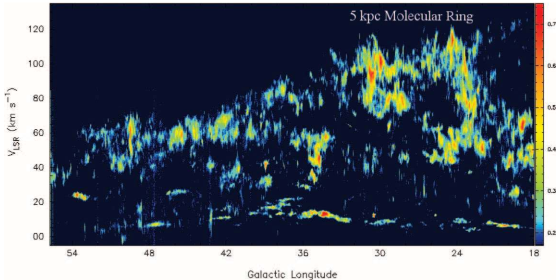
FIG. 3.—Position-velocity ( l - v ) diagram of GRS ^{13}\text{CO} emission, made by averaging over all Galactic latitudes ( |b| < 1^\circ ). Clearly evident are the large-scale Galactic features especially the molecular ring (the approximate location is marked). The image units are in K.
