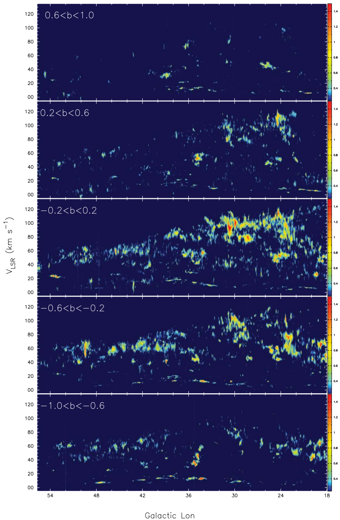
FIG. 4.—Position-velocity ( l - v ) diagram of GRS ^{13}\text{CO} emission averaged over five ranges in Galactic latitude. The latitude coverage of each image is labeled. The image units are in K.
