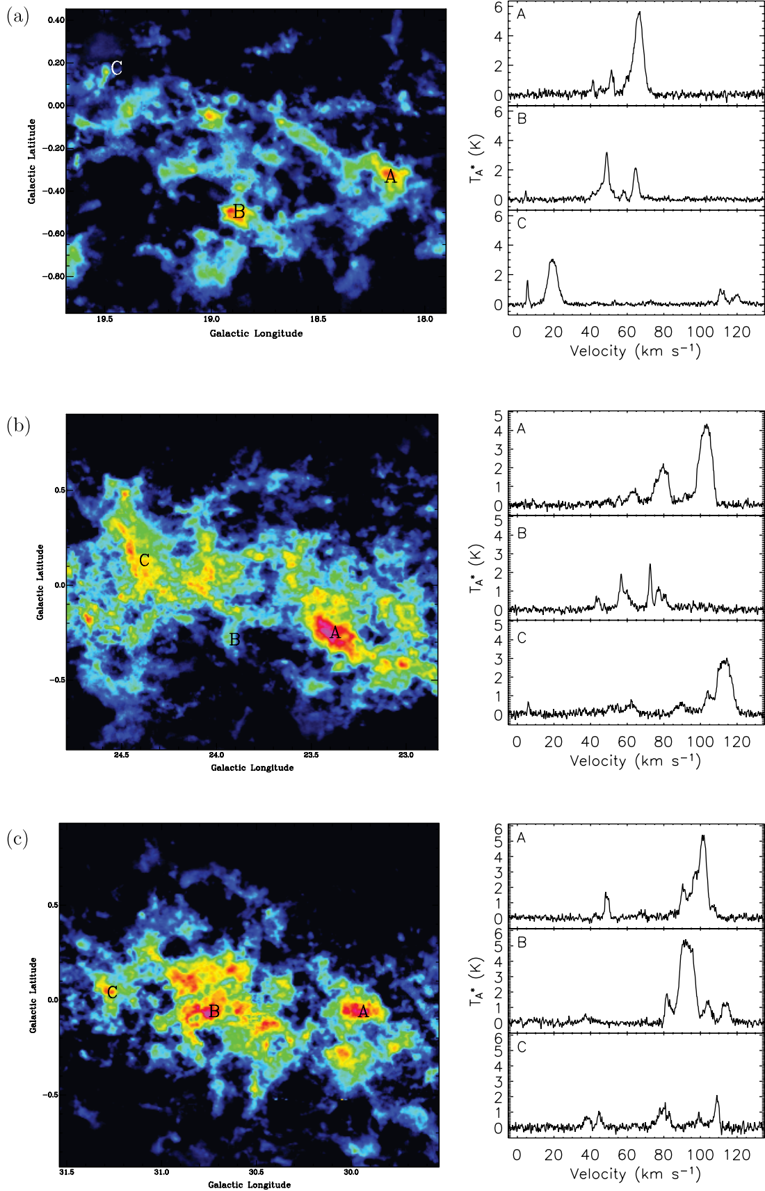
FIG. 12.—Integrated intensity images and sample spectra toward five regions within the GRS. The spectra typically show several distinct velocity components, an indication that several distinct molecular clouds lie along the line of sight. The location of each spectrum within the region is labeled on the image (A, B, and C). The transfer function is such that the following colors correspond to the following integrated intensities: black , 1 \text{K km s}^{-1} ; green , 20 \text{K km s}^{-1} ; red , 45 \text{K km s}^{-1} ; and white , 100 \text{K km s}^{-1} .
