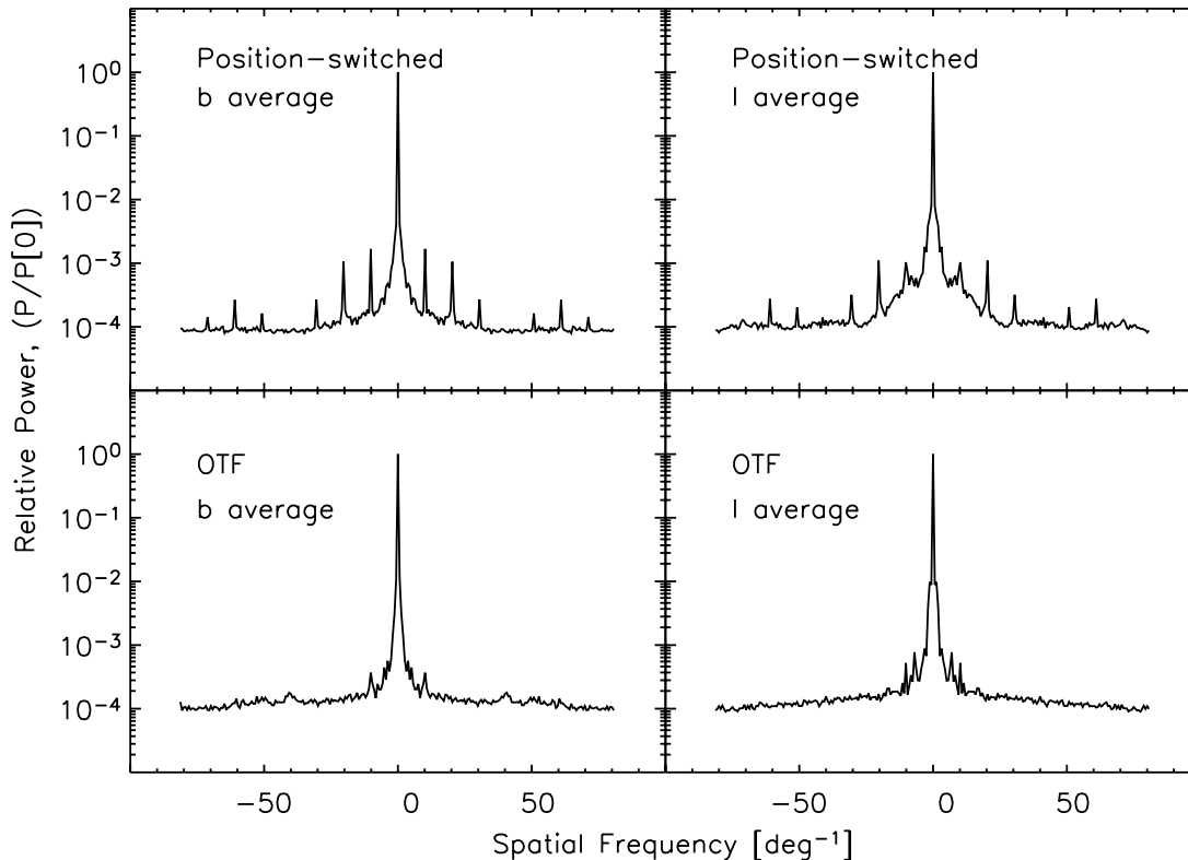
FIG. 11.—Power spectra of Fig. 10 averaged over Galactic latitudes ( left ) and longitudes ( right ). Peaks in this figure represent the correlated noise at certain spatial frequencies. For the position-switched data, the peaks in both directions correspond to multiples of the array size. In contrast, the OTF data show smaller correlated noise, and also a small peak at \sim 40 \text{ deg}^{-1} in the latitude plot due to the sharing of “off” positions in the scanning direction.
