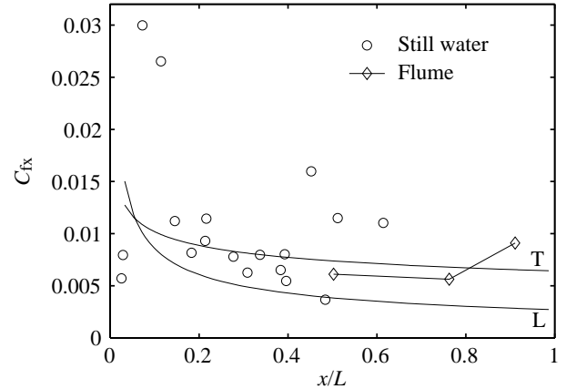
Fig. 10. Local friction coefficients, C_{fx} , representing 18 scup boundary layer realizations compiled from five still-water trials at swimming speeds of 10–40 \text{cm s}^{-1} (circles). Each point represents data from one boundary layer realization. The lines labeled ‘T’ and ‘L’ are flat-plate friction for turbulent and laminar boundary layer flow, respectively, with no streamwise pressure gradient. The whole-cycle-averaged local friction for scup swimming at 30 \text{cm s}^{-1} in the flume (Fig. 8A) is included and denoted by diamonds connected by solid lines. Sequences displaying incipient separation, i.e. C_{fx}=0 , were not included. Error bars are omitted for clarity. The uncertainty in C_{fx} is \pm 31\% . x , position along the body; L , body length.
