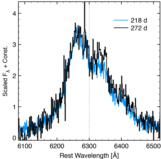
Figure 14. Late-time emission of [O I] \lambda\lambda 6300, 6364 in SN 2012ap between day 218 and 272. Emission redward of 6300 \text{ \AA} increases with time.
