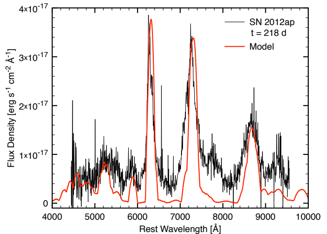
Figure 15. Late-time optical spectrum of SN 2012ap obtained 2012 September 23 ( t = 218 \text{ d} ; black) and our model fit (red).
