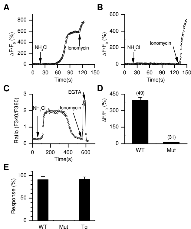
Figure 7 CATSPER1 is required for the NH 4 Cl-induced [Ca 2+ ] i rise in mouse sperm. (A-C) Representative responses to 20 mM NH 4 Cl in sperm head from a wild-type (A), a Catsper1 null (B), and transgenic sperm expressing an EGFP-CATSPER1 fusion protein on the Catsper1 null background (C). Ionomycin (10 μM, A-C) and EGTA (50 mM) were applied as control stimuli. (D) Averaged ΔF/F 0 changes induced by 20 mM NH 4 Cl in wild-type (WT) and Catsper1 null (Mut) sperm. Numbers of analyzed cells are in parentheses. (E) Percentages of sperm responsive to NH 4 Cl application in WT (n = 7 imaging runs; 3 mice, 56 cells), Catsper1 null (Mut; n = 7; 3 mice, 31 cells), and the Catsper1 mutant rescued with the EGFP-CatSper1 transgene (Tg; n = 7; 2 mice, 31 cells). Cells from Tg mice were imaged with Fura-2 and the others were imaged with Fluo-4.
