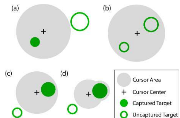
Figure 1. (a) Area cursors ease selection with larger hotspots than point cursors. (b) Isolating the intended target is difficult when the area cursor encompasses multiple possible targets. (c) The bubble cursor solves the problem in (b) by changing its size dynamically such that only the target closest to the cursor centre is selected. (d) The bubble cursor morphs to encompass a target when the basic circular cursor cannot completely do so without intersecting a neighboring target. Note that the same legend is used for Figures 1 to 5.
