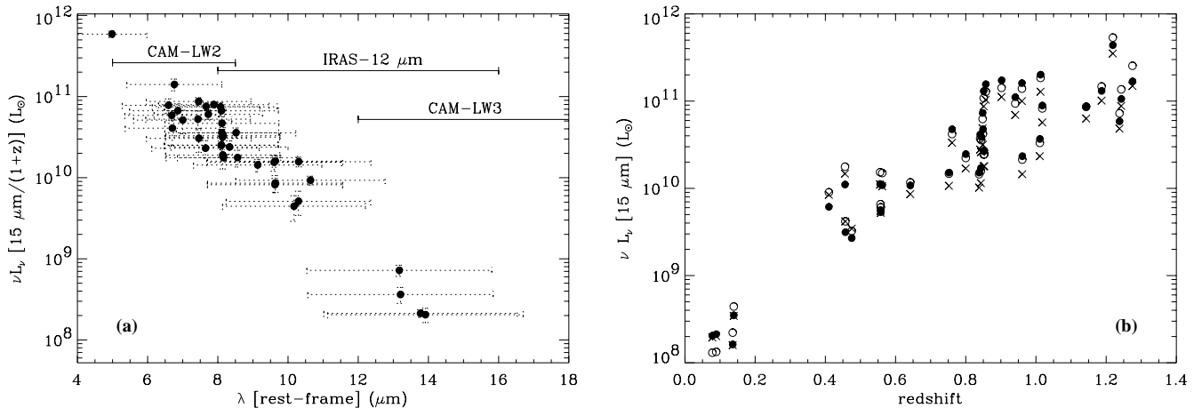
Fig. 7. Rest-frame MIR luminosity of ISOCAM-HDFN galaxies. a) luminosity of ISOCAM galaxies at \lambda_{\text{rf}} = 15/(1+z)\mu\text{m} as a function of \lambda_{\text{rf}} . The dotted lines represent the redshifted LW3 (12–18 \mu\text{m} ) band. b) rest-frame 15 \mu\text{m} luminosity ( \nu L_{\nu} ) versus redshift estimated with three different techniques: M 82 SED (crosses), “closest filter” (filled dots) and “multi-template” (open dots).
