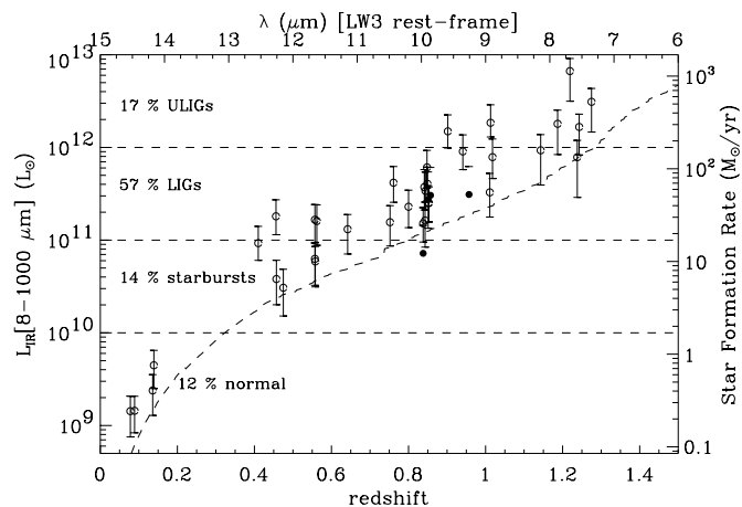
Fig. 8. L_{\text{IR}}[8-1000 \mu\text{m}] and star formation rate (SFR) versus redshift and \lambda_{\text{rf}} for the ISOCAM-HDFN galaxies ( S_{15} \geq 0.1 mJy). The 15 \mu\text{m} completeness limit of 0.1 mJy is materialized with a dashed line. Only the left axis is meaningful for the five AGNs (filled dots, Sect. 5.2). HDFN_PS3_6a (no spectroscopic redshift) is not included.
