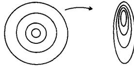
FIGURE 1b. Diffeo after lift.
