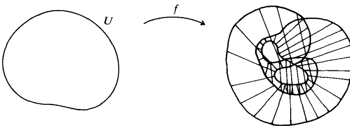
FIGURE 8. A locally injective map of one ball onto another.
