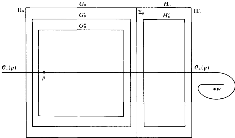
FIGURE 9. F_0 divided into subflowboxes.
