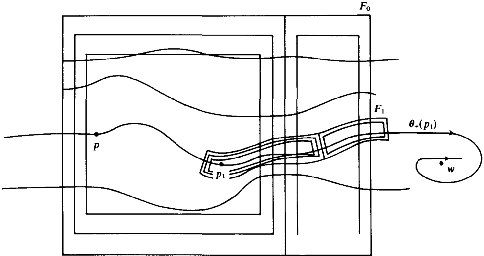
FIGURE 10. F_1 meeting F_0 , with X_0 -flow curves shown.
