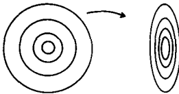
FIGURE 1a. Diffeo before lift.
