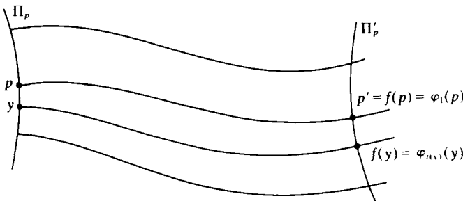
FIGURE 3. The Poincaré map and flowbox F .
