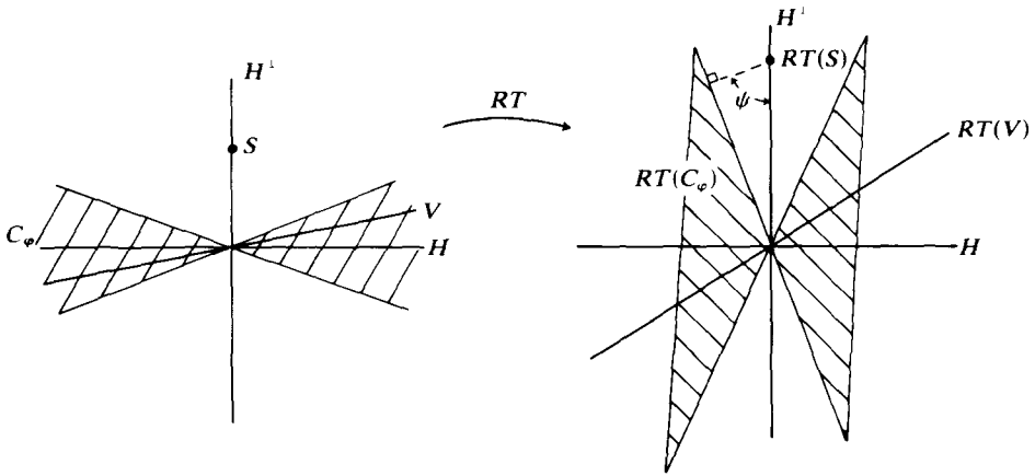
FIGURE 7. Cones mapped by RT .
