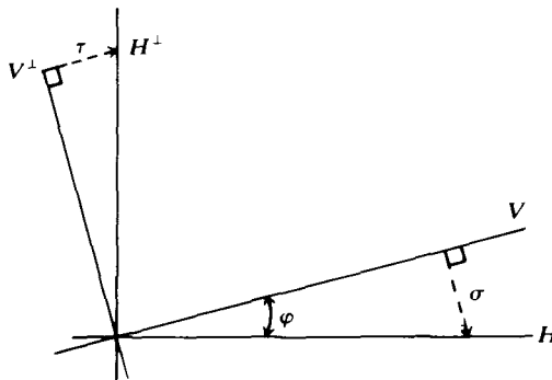
FIGURE 6. \mathbb{R}^m = H \oplus H^\perp = V \oplus V^\perp , \varphi = \angle(V, H) .
