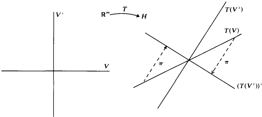
FIGURE 4. The V-altitude A = \pi \circ T/V .
