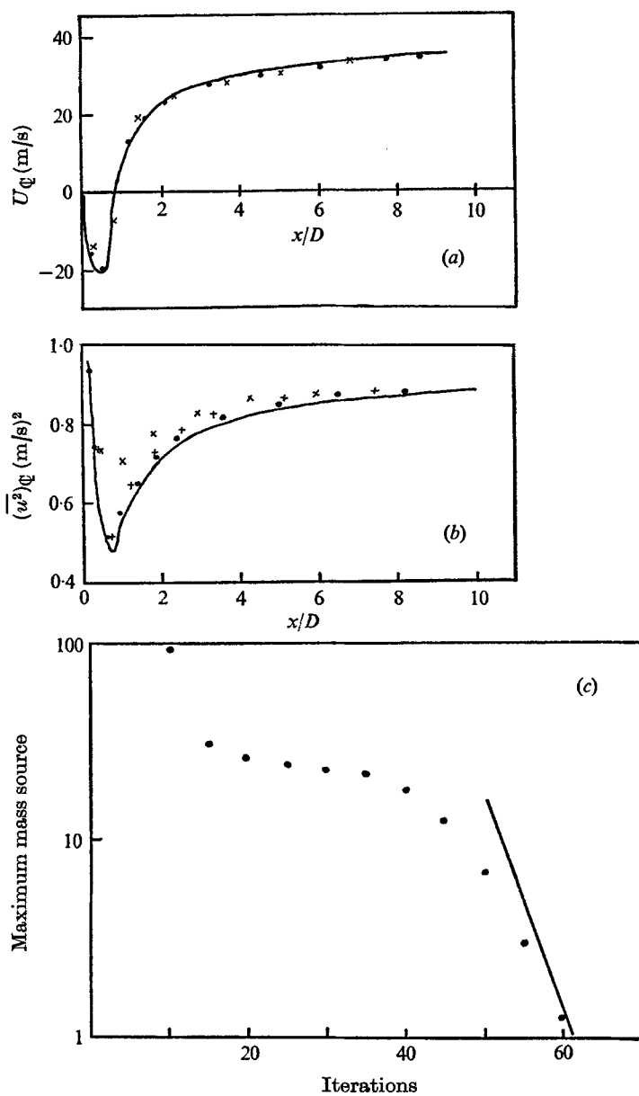
FIGURE 3. Solution-algorithm test calculations. (a) U_q vs. x/D . (b) (u^2)_q vs. x/D . (c) Maximum mass source vs. number of iterations. (a), (b) \times , 10 \times 10 grid; +, 14 \times 14 grid; \bullet , 18 \times 18 grid; —, 26 \times 26 grid.
