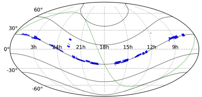
Figure 1. Geometry of the CFEPS discovery blocks. The R.A. and decl. grid is indicated with dotted lines. The black solid curves show constant ecliptic latitudes of -60^\circ , -30^\circ , 0^\circ , 30^\circ , 60^\circ from bottom to top. The remaining curve indicates the plane of the Milky Way.
