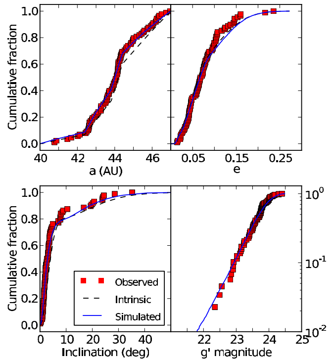
Figure 6. CFEPS+pre objects (red solid squares) compared to our main-belt model’s distribution in a (upper left), e (upper right), i (lower left), and g magnitude (lower right) distributions when the intrinsic (dashed line) are observed through the CFEPS Survey Simulator (resulting thin solid lines). The model used here is the one described in Section 5.1, with values of the parameters corresponding to our nominal case (see Section 5.1.2).
