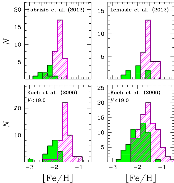
Fig. 5.— The metallicity distribution of the three spectroscopic samples. The top panels show the high-resolution samples: Fabrizio et al. (2012, 44 stars, left) and Lemasle et al. (2012, 35 stars, right). In the lower panels, the medium-resolution sample from Koch et al. (2006) was split in two subgroups: stars with V < 19 mag (71, bottom left), and stars with V \geq 19 mag (141, bottom right).
