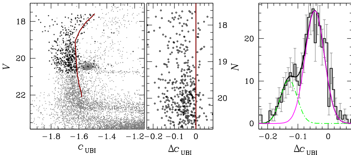
FIG. 3.— Same as Figure 2, but in this case the open circles in the left panel mark 413 RGB stars with radial velocity consistent with that of Carina, selected from the sample of Fabrizio et al. (2011). In the right panel, the presence of a double peak in the \Delta c_{U,B,I} distribution is confirmed.
