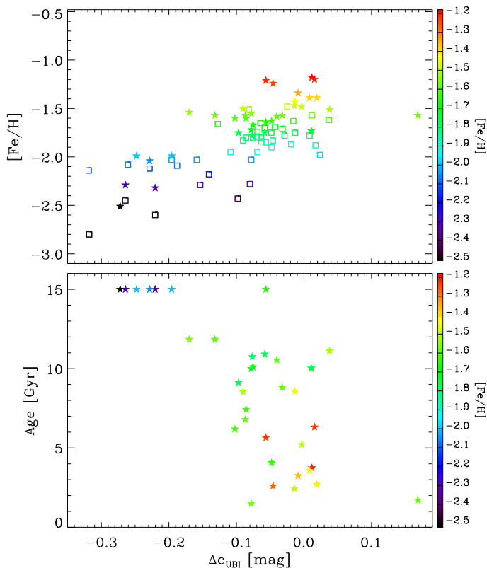
FIG. 11.— Iron abundance (top panel) and age (bottom) from Lemasle et al. (2012) as a function of the \Delta c_{U,B,I} index. The colour code used in both panels accounts for the metallicity of the 35 stars, and is the same used in the top panel of Fig. 10. The error bars account for the photometric error of our photometry and the uncertainties provided by Lemasle et al. (2012) on their age and metallicity determinations.
