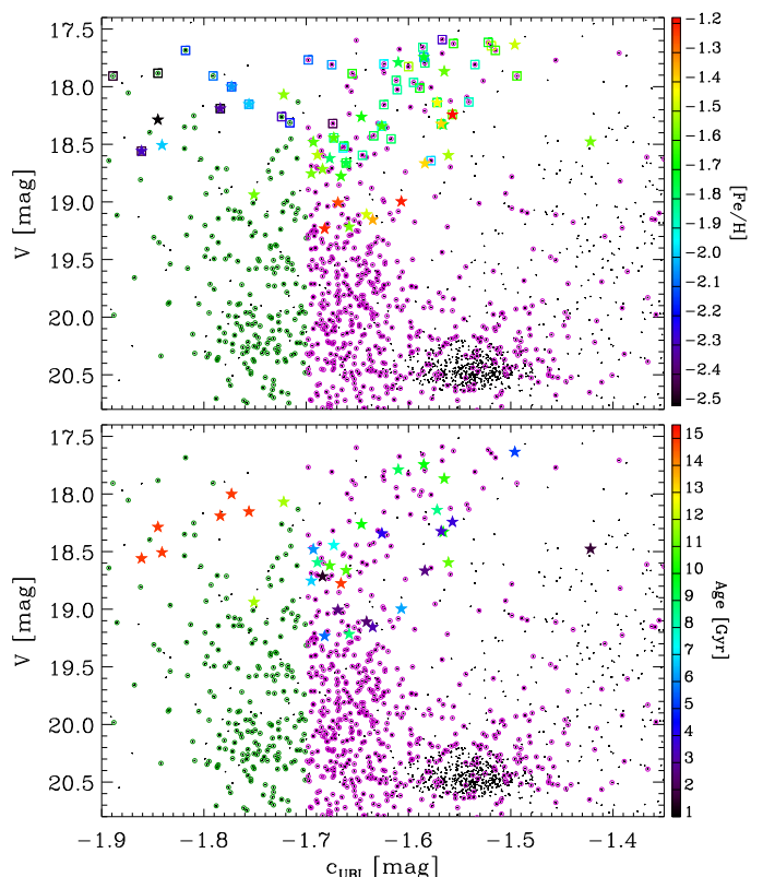
FIG. 10.— V - c_{\text{U,B,I}} diagram for bright Carina stars. The green and magenta circles show the separation at c_{\text{U,B,I}} = -1.70 mag performed in Fig. 6. The starred symbols highlight the 35 stars from Lemasle et al. (2012). The colour code used for these symbols, reproduced on the right of both panels, displays the iron content (top) and age (bottom) determined by Lemasle et al. (2012).
