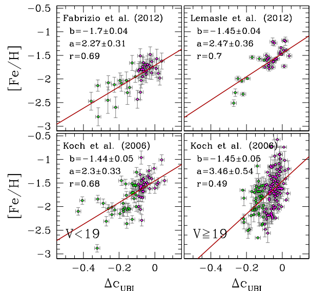
FIG. 7.— Same as Fig. 6, but in this case green and magenta symbols show stars with \Delta c_{\text{U,B,I}} < -0.1 mag and \Delta c_{\text{U,B,I}} > -0.1 mag, respectively. The plot demonstrates that the selection criterium does not affect the derived conclusions.
