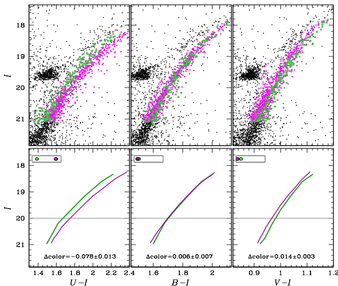
FIG. 9.— Top - I versus U - I , B - I , V - I CMDs zoomed in the RGB region, with stars from the two RGB selected in the \Delta c_{\text{U,B,I}} are highlighted in green (old population) and magenta (intermediate-age). Bottom - Ridge lines of the two populations. Note the change in the relative position for decreasing colour baseline. The mean colour difference with respect of the green line at magnitude I = 20 mag is labeled, and illustrated by the coloured points on the top-left corner of each panel.
