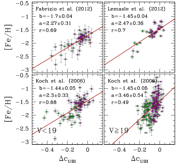
FIG. 6.— Top - Correlation between the c_{\text{U,B,I}} colour and the iron content of stars for the high-resolution samples. Bottom - The same is shown also for the Koch et al. (2006) sample. The slope of the relation changes according to the luminosity of the sample. See text for details. Green and magenta symbols indicate stars with c_{\text{U,B,I}} < -1.70 mag and c_{\text{U,B,I}} > -1.70 mag, respectively, as in Fig. 5 and Fig. 6.
