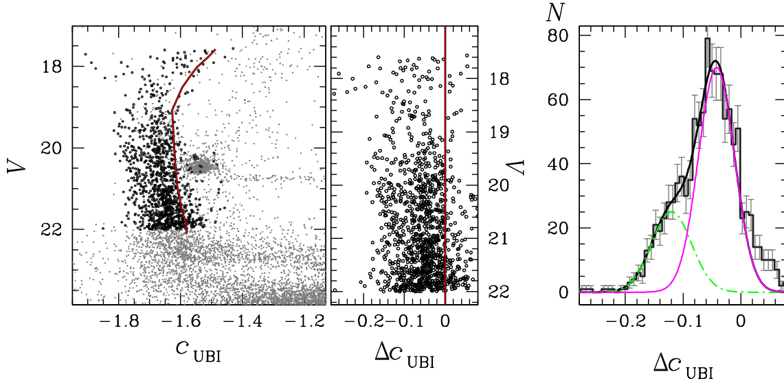
FIG. 2.— Left ) The sample of RGB stars adopted to identify substructures in the RGB of Carina are shown as black open circles (1134 stars). The red line shows our adopted right envelope of the sequence. Center - the Carina RGBs, rectified to the red line. For each star we display the \Delta c_{U,B,I} index, the colour difference with respect to the reference red line. Right - Histogram of \Delta c_{U,B,I} , with gaussian kernels superimposed. The overall distribution can be well represented by two gaussian components.
