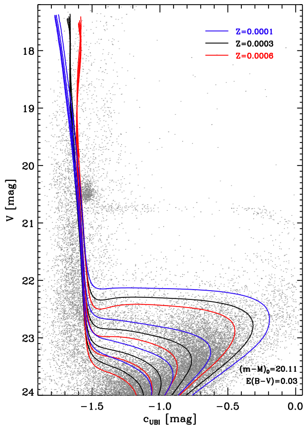
FIG. 8.— Comparison with theoretical isochrones from the BaSTI database in the (M_V, c_{U,B,I}) plane. For the three metallicity labeled, isochrones with age between 4 and 13 Gyr, in steps of 3 Gyr, are plotted.
