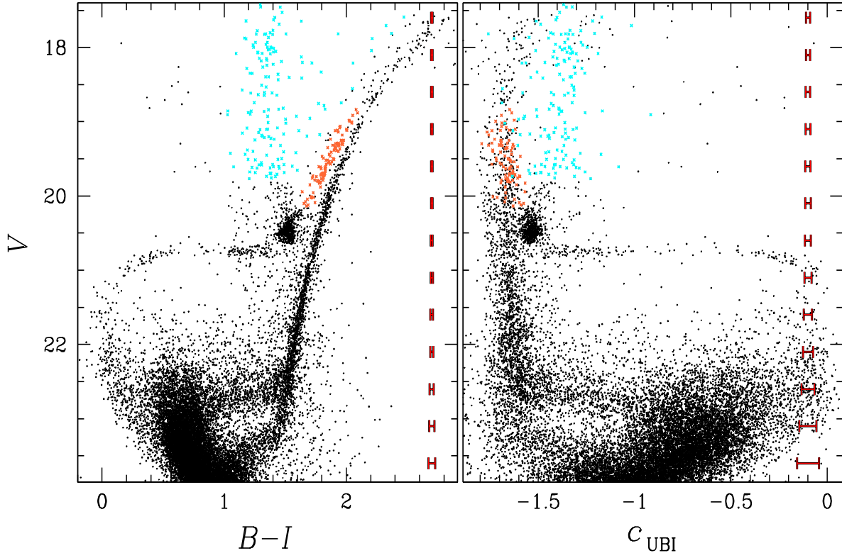
FIG. 1.— Left - (V, B-I) CMD of Carina stars, based on the photometry presented in Bono et al. (2010). Bright field stars are highlighted in cyan, while orange symbols show the Carina AGB stars; Right - (V, c_{U,B,I}) plane, where the RGBs of the old and intermediate-age populations largely split.
