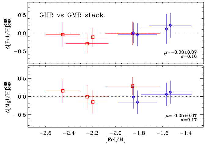
Fig. 9. Comparison of Fe I and Mg I abundances between stacked Giraffe HR and LR08 spectra, \Delta[X/\text{H}] = [X/\text{H}]_{\text{GHR}} - [X/\text{H}]_{\text{GMR}} .
