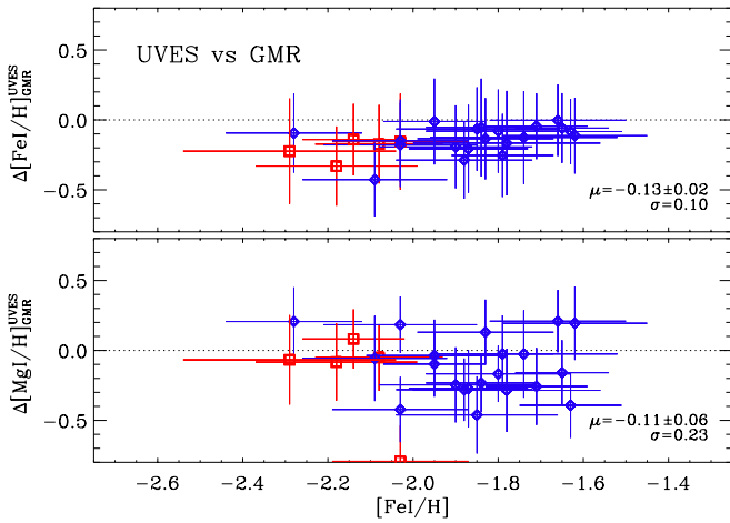
Fig. 8. Comparison of Fe I and Mg I abundances between UVES and individual Giraffe MR spectra, \Delta[X/\text{H}] = [X/\text{H}]_{\text{UVES}} - [X/\text{H}]_{\text{GMR}} .
