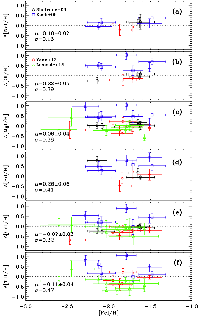
Fig. 6. Comparison of UVES abundances with the literature data samples indicated, \Delta[X/H] = [X/H]_{UVES} - [X/H]_{Other} .
