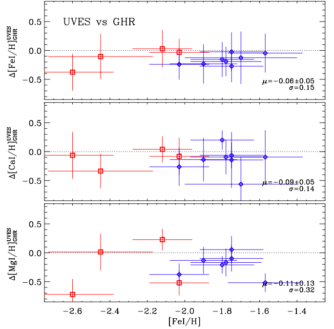
Fig. 7. Comparison of Fe I, Ca I, and Mg I abundances between UVES and individual Giraffe HR spectra, \Delta[X/H] = [X/H]_{UVES} - [X/H]_{GHR} . Red squares and blue diamonds show abundances of old and intermediate-age stars.
