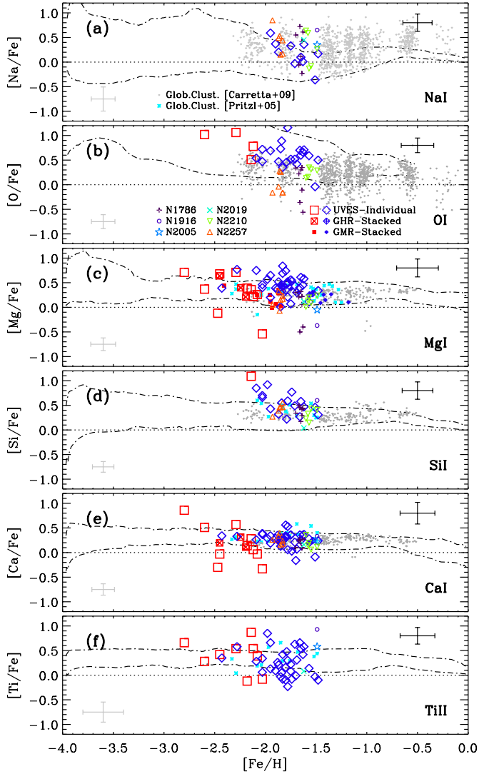
Fig. 13. Element abundances as functions of [Fe/H] for Galactic and some LMC GCs. Red squares and blue diamonds show abundances of old and intermediate-age Carina stars. The small cyan asterisks are mean abundances for Galactic GCs from Pritzl et al. (2005). The colored small symbols are data for LMC clusters from Mucciarelli et al. (2010, NGC 1786, NGC 2210, and NGC 2257) and Colucci et al. (2012, NGC 1916, NGC 2005, and NGC 2019). The gray dots are individual abundances for 19 Galactic GCs from Carretta et al. (2009a,b, 2010a). The gray error bars in the bottom left corner of each panel show the mean abundance errors in GCs. The two dot-dashed lines show the limiting positions of the Milky Way halo stars Frebel (2010).
