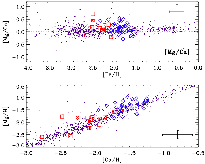
Fig. 18. Top panel : ratio [Mg/Ca] as a function of [Fe/H] for Carina as compared to MW halo stars. Symbols and colors are the same as in Fig. 11. The abundances of [Mg/H] and [Ca/H] are compared in the bottom panel , where the dashed line shows the bisector of the plane.
