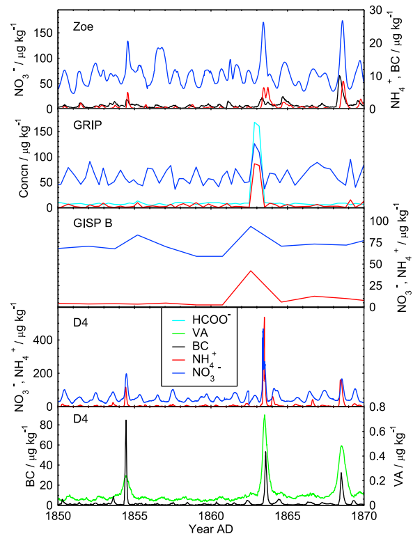
Figure 4. Chemical records for Greenland ice cores for the period 1850–1870. In each case nitrate is in blue, ammonium in red, black carbon (BC) in black, vanillic acid (VA) in green, formate in turquoise. Note the different scales on the y-axis for each record.
