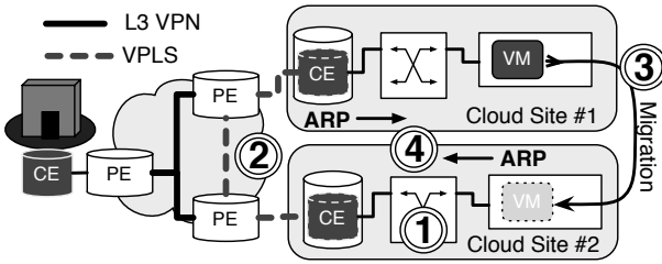
Figure 3: WAN migration using VPLS to move across sites.
