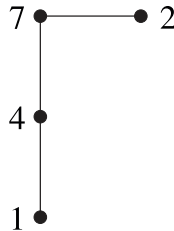
FIG. 2. The Hasse diagram of the poset P_{(3,5)} .
