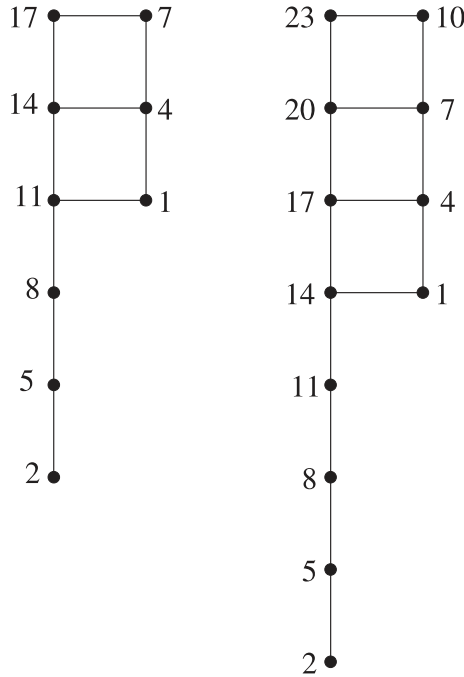
FIG. 3. The Hasse diagrams of P_{(3,10)} (on the left) and P_{(3,13)} .
