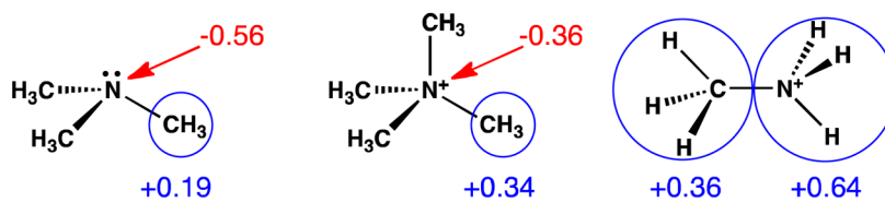
Figure 2. Charge distributions in representative structures. HF-6-31G**, natural charge distributions.
