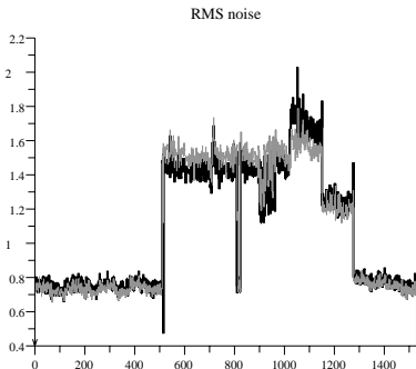
Figure 5. Noise (dark) and Dnoise (light) on a stave. Channels 1-512 and 1350-1536 are unbonded, channels 513-1290 are bonded to two sensors (full load). Channels 1050-1290 are damaged, resulting in excess leakage current and noise. Channels 1291-1349 are bonded to one sensor. Two-sensor noise is about 1200 electrons.
