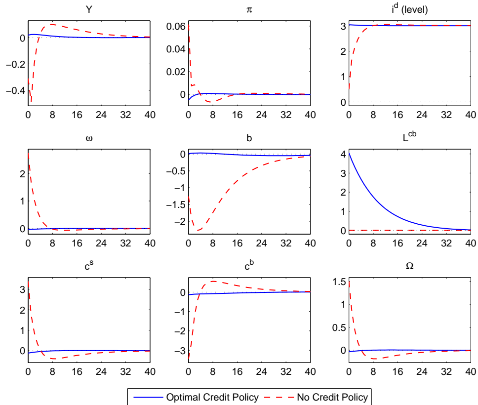
Figure 10: Impulse responses under optimal credit policy compared to those under a policy of “Treasuries only,” with the same disturbance as in Figure 9, but under optimal interest-rate policy. Again \tilde{\Xi}^{cb} is exactly equal to the steady-state critical threshold.
