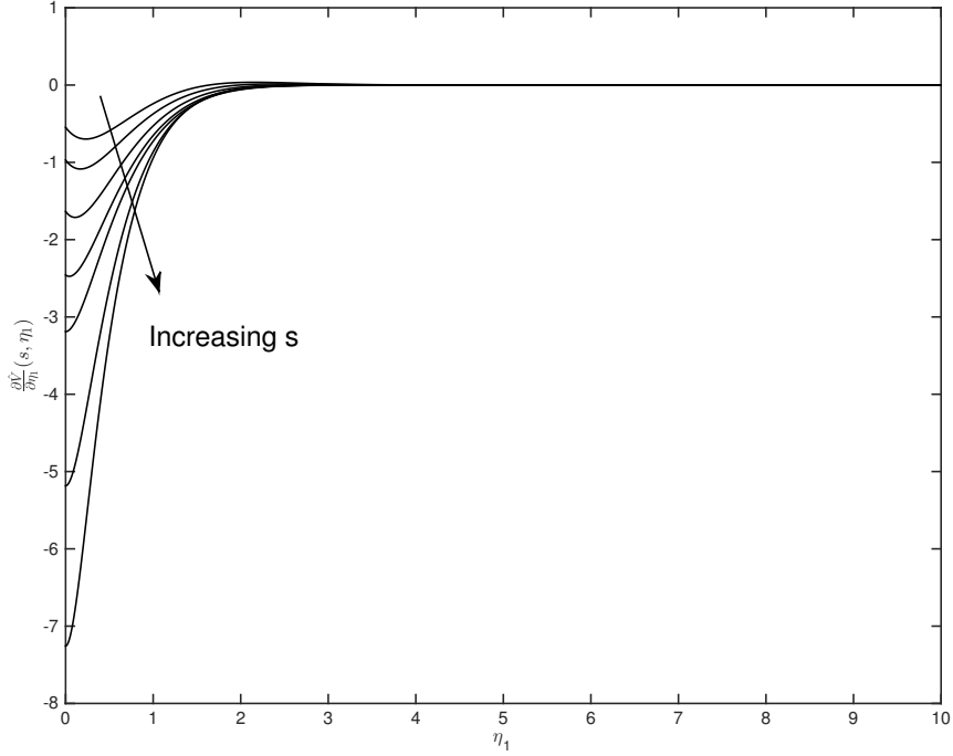
FIGURE 3. Plots of \frac{\partial \tilde{V}}{\partial \eta_1}(s, \eta_1) for a slender rotating cone with \psi = 15^\circ , s = 1.5, 2, 3, 4, 5, 10, 16 .
