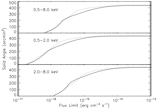
FIG. 14.—Survey solid angle as a function of the flux limit for the full ( top ), soft ( middle ), and hard ( bottom ) bands, determined following § 4. Data are plotted as solid curves for the \approx 2 Ms CDF-S and as dotted curves for the \approx 2 Ms CDF-N. The flux limits at the average aim point of the CDF-S are \approx 7.1 \times 10^{-17} ergs \text{cm}^{-2} \text{s}^{-1} (full band), \approx 1.9 \times 10^{-17} ergs \text{cm}^{-2} \text{s}^{-1} (soft band), and \approx 1.3 \times 10^{-16} ergs \text{cm}^{-2} \text{s}^{-1} (hard band).
