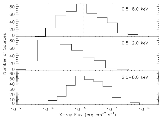
FIG. 8.—Histograms showing the distributions of X-ray fluxes for sources in the main Chandra catalog in the full (top), soft (middle), and hard (bottom) bands. Sources with upper limits have not been included in this figure. The vertical dotted lines indicate the median fluxes of 1.3 \times 10^{-15} , 2.5 \times 10^{-16} , and 1.7 \times 10^{-15} ergs \text{cm}^{-2} \text{s}^{-1} for the full, soft, and hard bands, respectively.
