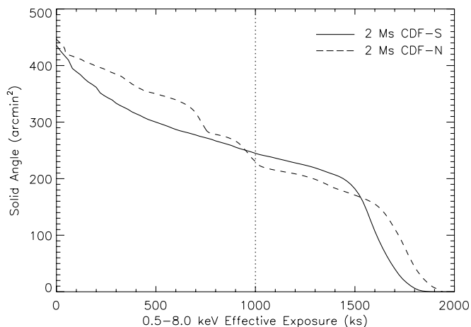
FIG. 3.—Amount of survey solid angle having at least a given amount of full-band effective exposure for the \approx 2 Ms CDF-S ( solid curve ). The maximum exposure is \approx 1.884 Ms. The vertical dotted line shows an effective exposure of 1 Ms. About 245 arcmin 2 ( \approx 56\% ) of the CDF-S survey area has >1 Ms effective exposure. Corresponding data from the \approx 2 Ms CDF-N (A03) are plotted as a dashed curve for comparison.
