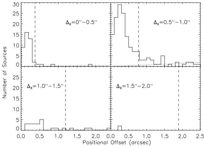
FIG. 6.—Histograms showing the distributions of positional offset for sources in the main Chandra catalog that were matched to WFI R -band optical sources with R \leq 24 within 2.5'' . X-ray sources were divided into four bins based on their positional uncertainties estimated using eq. (1): 0''\text{--}0.5'' , 0.5''\text{--}1.0'' , 1.0''\text{--}1.5'' , and 1.5''\text{--}2.0'' . The vertical dashed line indicates the median positional uncertainty for X-ray sources in each bin. Dotted lines show how many random R \leq 24 optical sources are expected as a function of the positional offset. Less than 20% of the optical counterparts lie beyond the median X-ray positional uncertainties in all cases.
