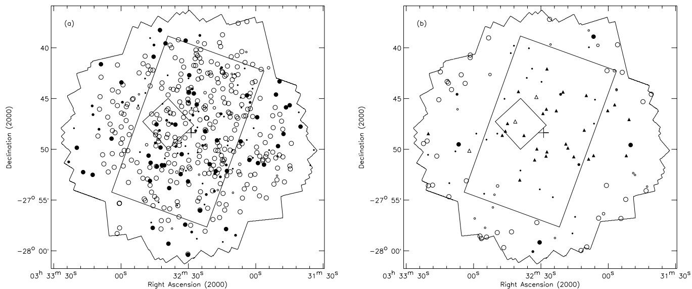
FIG. 10.—Positions of the sources in (a) the main Chandra catalog and (b) the supplementary Chandra catalogs. Circles represent X-ray sources in (a) the main Chandra catalog and (b) the supplementary CDF-S plus E-CDF-S Chandra catalog. Open circles represent X-ray sources that were previously detected in (a) the main catalogs of G02 or A03 and (b) the main catalogs of G02, A03, or L05. Filled circles represent new sources. Sizes indicate the maximum detection significance corresponding to wavdetect false-positive probability detection thresholds of 1 \times 10^{-8} (large circles), 1 \times 10^{-7} (medium circles), and 1 \times 10^{-6} (small circles). Sources in the optically bright catalog are shown as open triangles (previously detected in the main catalog of A03) and filled triangles (new sources) in (b). For sources in the CDF-S plus E-CDF-S catalog, their detection significances are preferentially higher near the edge of the field due to the contribution of the E-CDF-S exposure. The regions and the plus sign have the same meaning as those in Fig. 1.
