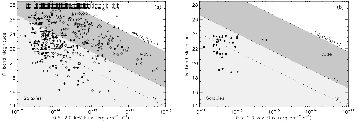
FIG. 12.—WFI R -band magnitude vs. soft-band flux for X-ray sources in (a) the main catalog and (b) the supplementary optically bright catalog. Open circles represent X-ray sources that were detected in the main catalogs of G02 or A03. Filled circles represent new sources. Sources without an optical counterpart are plotted as upward arrows. Diagonal lines indicate constant flux ratios. The shaded areas show the approximate flux ratios for AGNs (dark gray) and galaxies (light gray).
