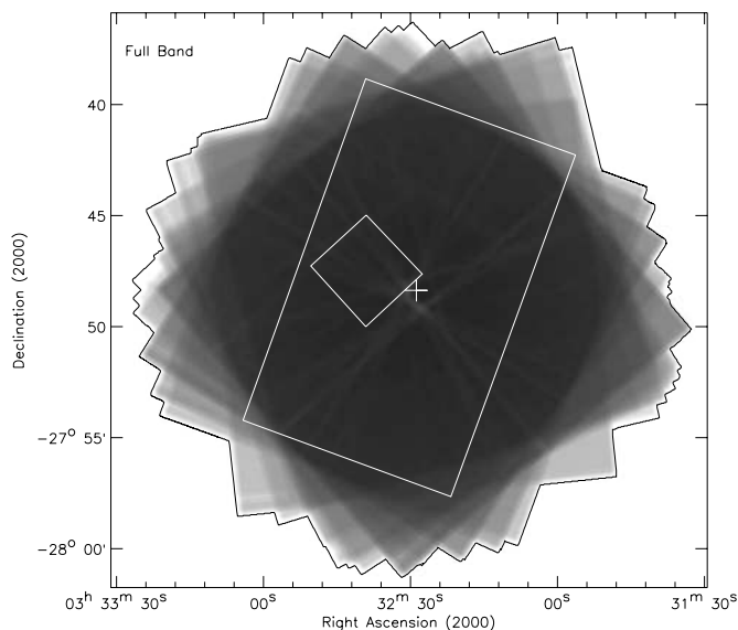
FIG. 2.—Full-band (0.5–8.0 keV) exposure map of the \approx 2 Ms CDF-S. The darkest areas represent the highest effective exposure times (the maximum value is 1.884 Ms). The gray scales are logarithmic. The regions and the plus sign have the same meaning as those in Fig. 1.
