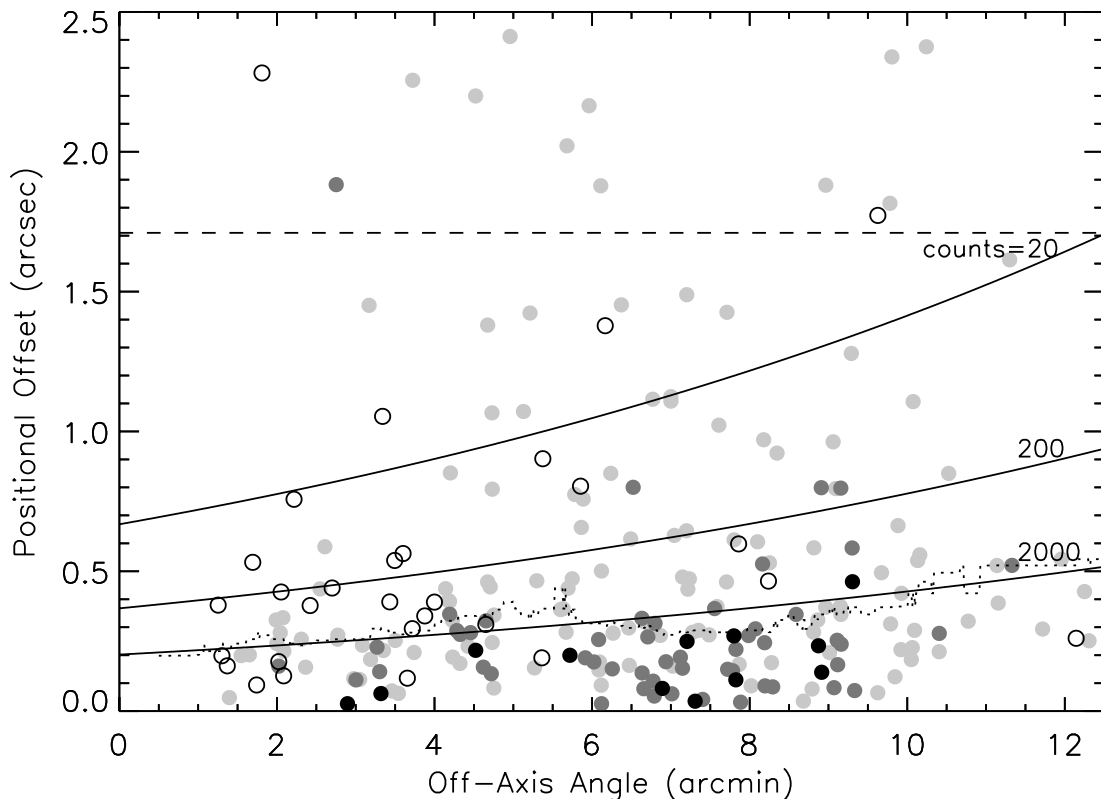
FIG. 5.—Positional offset vs. off-axis angle for sources in the main Chandra catalog that were matched to WFI R -band optical sources with AB magnitude R \leq 24 to within 2.5'' . Black, dark gray, light gray, and open circles represent Chandra sources with \geq 2000 , \geq 200 , \geq 20 , and < 20 counts in the energy band where the source position was determined, respectively. The dotted curve shows the running median of all sources in bins of 2' . The median offset of the expected false matches ( \approx 1.71'' ) is indicated by the dashed line. These data were used to derive the \approx 85\% confidence-level positional uncertainties of the X-ray sources in the main catalog; see eq. (1). Three solid curves indicate the \approx 85\% confidence-level positional uncertainties for sources with counts of 20, 200, and 2000. The numbers of black, dark gray, and light gray circles lying below/above their corresponding solid curves are 11/1, 48/4, and 116/20, respectively. Note that sources with more than 20 or 200 counts will have expected positional uncertainties smaller than those indicated by the corresponding solid curves.
