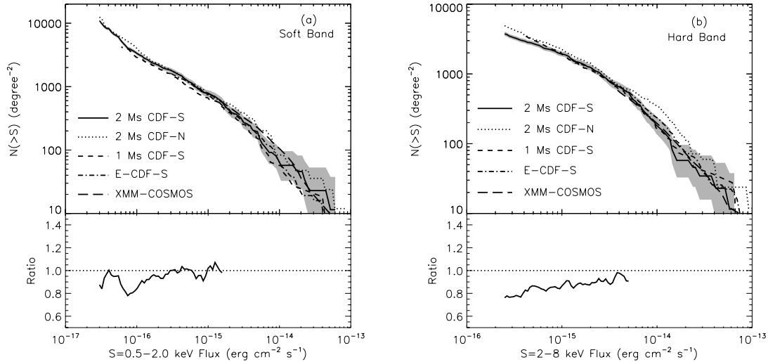
FIG. 15.— Top : Number of sources, N(>S) , brighter than a given flux, S , for the (a) soft band and (b) hard band. The \approx 2 Ms CDF-S data are plotted as black solid curves with the 1\sigma errors plotted as gray shaded areas. The cumulative number counts were computed using 428 X-ray sources in the main Chandra catalog that are located within 10' of the average aim point and have been corrected for incompleteness and flux bias. Also shown are the cumulative number-count results for the \approx 2 Ms CDF-N (dotted curves), the \approx 1 Ms CDF-S (dashed curves; Rosati et al. 2002), the \approx 250 ks E-CDF-S (dash-dotted curves; L05), and XMM-Newton observations in the COSMOS field (long-dashed curves; Cappelluti et al. 2007). The 2–10 keV fluxes in the \approx 1 Ms CDF-S and the COSMOS field were converted to 2–8 keV fluxes assuming a photon index \Gamma = 1.4 . Bottom : Ratio of the CDF-S to CDF-N cumulative number counts for the (a) soft band and (b) hard band. Ratios were calculated only for number counts that were derived from a sample of \geq 50 sources, since for smaller numbers of sources there are large statistical errors. This corresponds to soft-band fluxes \leq 1.5 \times 10^{-15} ergs \text{cm}^{-2} \text{s}^{-1} and hard-band fluxes \leq 5 \times 10^{-15} ergs \text{cm}^{-2} \text{s}^{-1} . [See the electronic edition of the Supplement for a color version of this figure.]
