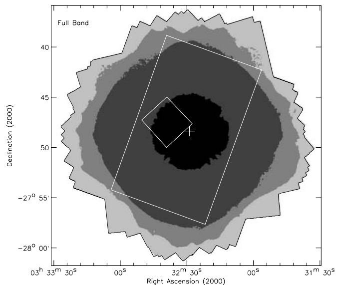
FIG. 13.—Full-band sensitivity map of the 2 Ms CDF-S. This sensitivity map has been created following § 4. The gray-scale levels (from black to light gray) represent areas with flux limits (in units of ergs cm -2 s -1 ) of <10^{-16} , 10^{-16} to 3.3 \times 10^{-16} , 3.3 \times 10^{-16} to 10^{-15} , and >10^{-15} , respectively. The regions and the plus sign have the same meaning as those in Fig. 1.
