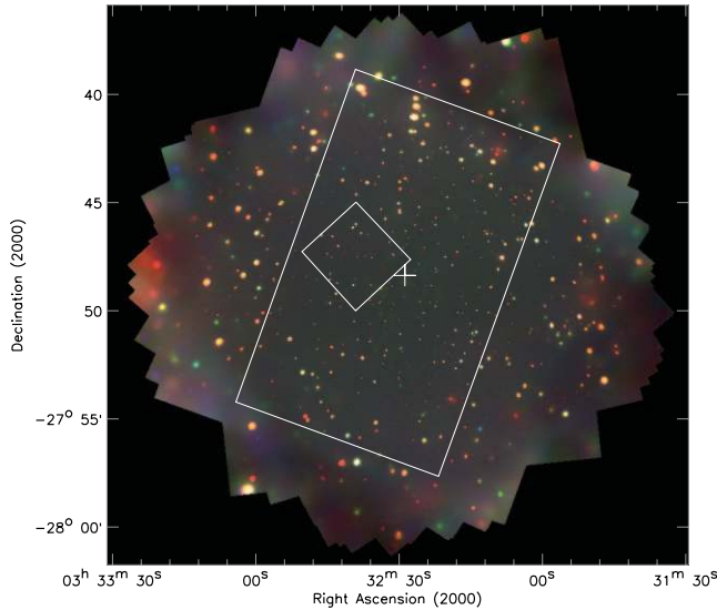
FIG. 4.— Chandra “false-color” image of the \approx 2 Ms CDF-S. This image is a color composite of the exposure-corrected adaptively smoothed images in the 0.5–2.0 keV (red), 2–4 keV (green), and 4–8 keV (blue) bands. The apparent smaller size and lower brightness of sources near the field center is due to the small PSF at that location. The regions and the plus sign have the same meaning as those in Fig. 1.
