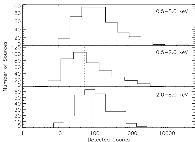
FIG. 7.—Histograms showing the distributions of detected source counts for sources in the main Chandra catalog in the full (top), soft (middle), and hard (bottom) bands. Sources with upper limits have not been included in these diagrams. The vertical dotted lines indicate the median numbers of counts in each band (see Table 3).
