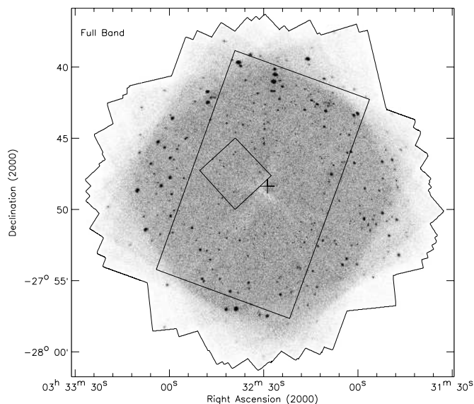
FIG. 1.—Full-band (0.5–8.0 keV) raw image of the \approx 2 Ms CDF-S. The gray scales are linear. The apparent scarcity of sources near the field center is largely due to the small PSF at that location (see Figs. 4 and 10 for clarification). The black outline surrounding the image indicates the extent of all the CDF-S observations. The large rectangle indicates the GOODS-S (Giavalisco et al. 2004) region, and the central square indicates the Hubble Ultra Deep Field (UDF; Beckwith et al. 2006) region. The plus sign near the center of the images indicates the average aim point, weighted by exposure time (see Table 1).
