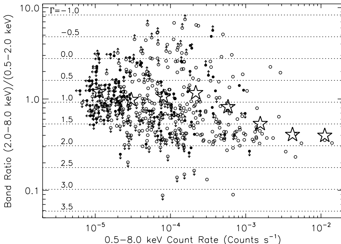
FIG. 11.—Band ratio vs. full-band count rate for sources in the main Chandra catalog. Open circles represent X-ray sources that were detected in the main catalogs of G02 or A03. Filled circles represent new sources. Plain arrows indicate upper or lower limits. Sources detected only in the full band cannot be plotted. The open stars show average band ratios as a function of full-band count rate derived from stacking analyses. Horizontal dotted lines show the band ratios corresponding to given effective photon indices; these were calculated using PIMMS.
