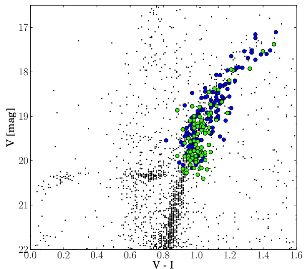
Fig. 2: Colour-magnitude diagram of the Sextans stars. The blue and green points are in as in Fig. 1. The black dots correspond to Sextans photometry taken with the CFH12K CCD camera at Canada-France-Hawaii Telescope (CFHT; Lee et al. 2003).
