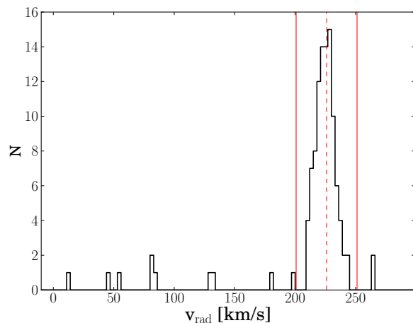
Fig. 3: Radial velocity distribution of our stars (black solid line). The dashed red line corresponds to the mean radial velocity from Battaglia et al. (2011) based on 174 probable members: v_{\text{sys, helio}} = 226.0 \pm 0.6 \text{ km/s} . The two solid red lines represent the \pm 3\sigma interval within which the membership zone is defined.
