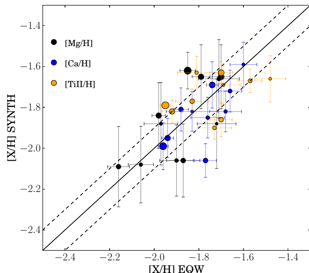
Fig. 9: Comparison between the abundances of three \alpha -elements derived by the EQW and SYNTH methods. The solid line traces the line of equality while the dashed lines indicate a variation by \pm 0.1 dex around this line.
