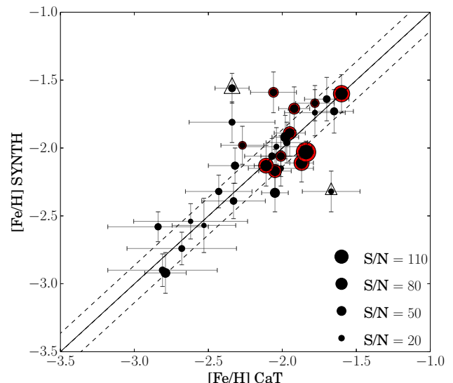
Fig. 6: Comparison between the CaT metallicity estimates and the [\text{Fe}/\text{H}] values derived from spectral synthesis (SYNTH). The size of the points is a function of the S/N of the spectra. The two stars S08-75 and S08-59, which have been discarded from further analysis (see text) are identified with triangles. We highlight in red the stars which have been independently analysed with a classical method based on equivalent widths and which are in Fig. 7.
