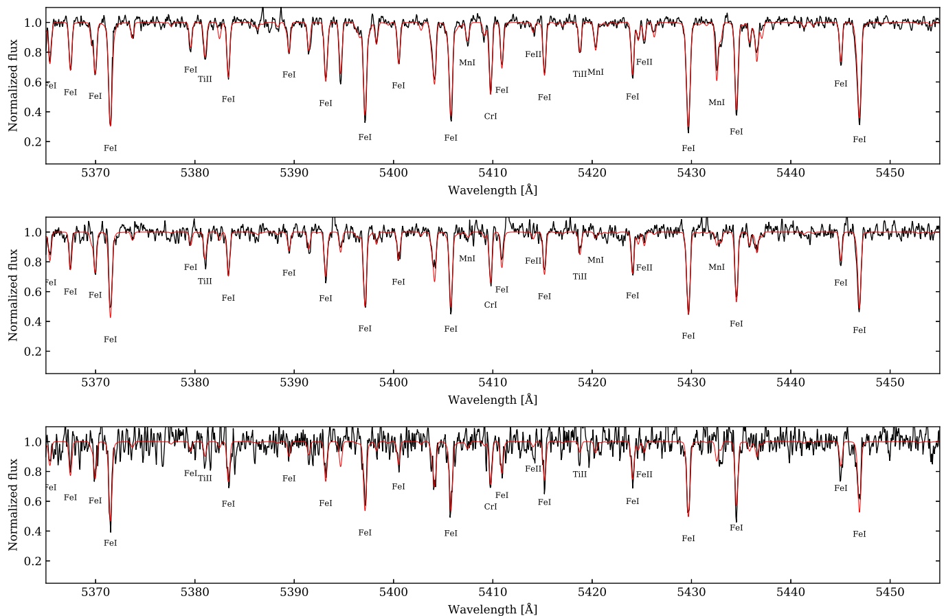
Fig. 4: Part of the HR10 spectrum of S08-6 (top), S08-242 (middle) and S05-67 (bottom) in black with their synthetic best fits over-plotted in red. A set of lines used in abundance determination are indicated for each star. The stars are ranked from top to bottom by decreasing signal-to-noise ratios: 83, 38, and 23.
