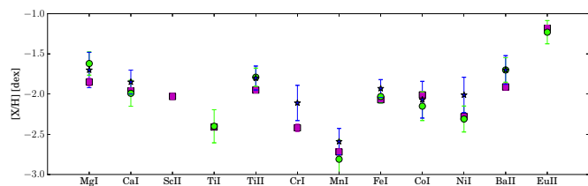
Fig. 10: Elemental abundances of the star S08-3. The green circles refer to this study, the blue stars come from Shetrone et al. (2001), and the magenta squares are from the EQW analysis.
