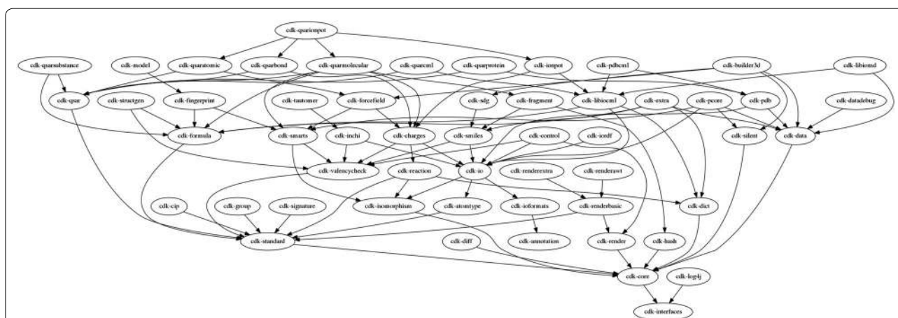
Fig. 7 Dependencies between CDK modules. Visualization of the dependencies between CDK modules. For example, the cdk-core depends on the cdk-interfaces module. A few higher level modules have been left out: cdk-builder3dtools, cdk-legacy, and cdk-depict
