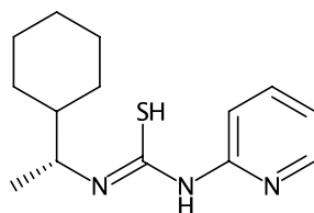
Fig. 6 Structure diagram generation for structures with double bond and tetrahedral stereochemistry
