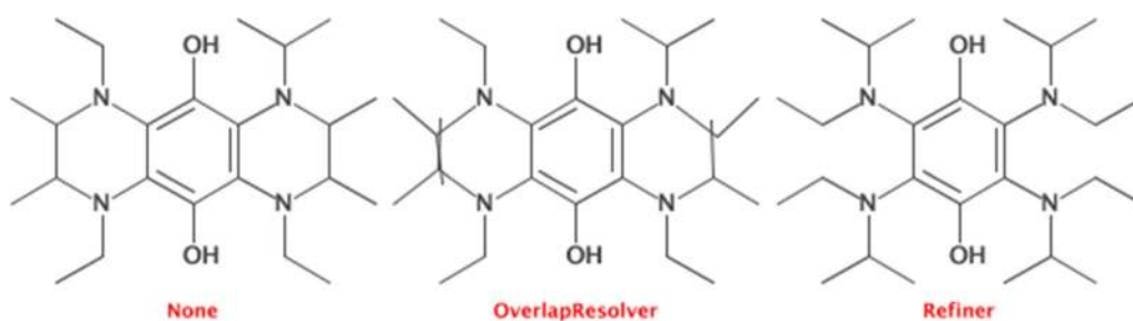
Fig. 5 The improved structure diagram generation has improved code to solve overlap. The original SDG code used general heuristics ( left ) and the OverlapResolver would fine tune the layout to ensure atoms would not be placed at the same location ( middle ). The new SDG algorithm is able to make more rigorous changes, making the final output must more pleasing ( right )
