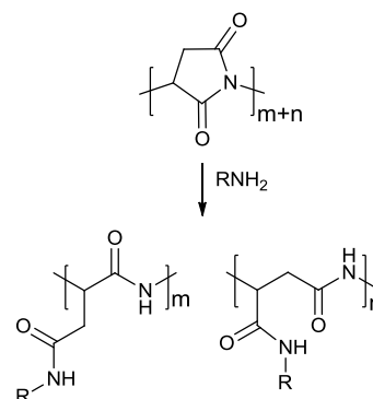
Scheme 2 Synthesis of polyaspartamides from polysuccinimide. 75
