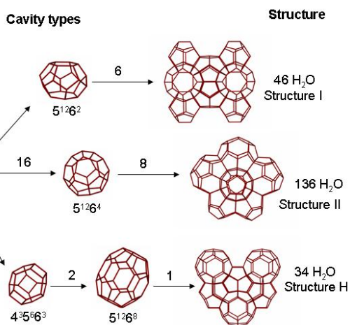
Fig. 2 Common clathrate hydrate structures (reproduced with permission from ref. 13 )
