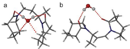
Fig. 15 DFT structures of (a) hydrogenated and (b) unsaturated dimeric model compounds derived from VCap showing binding to H 2 O (reproduced with permission from ref. 55 )
