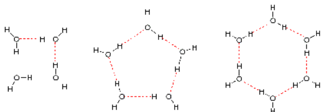
Fig. 1 Hydrogen bonded water motifs comprising the faces in clathrate hydrate cages (reproduced with permission from ref. 13 )
