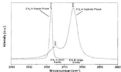
Fig. 11 Raman Spectra for \nu_1 of methane vapour incorporated in the structure I hydrate. Two peaks are seen for the hydrate phase, showing that CH 4 is incorporated into both cavities of the structure I hydrate (reproduced with permission from ref. 114 )
