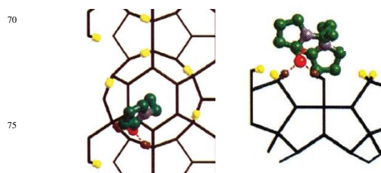
Fig. 14 Simulation result showing the formation of two hydrogen bonds between the pyrrolidone oxygen atom and hydrogen atoms on the hydrate surface (brown = H of hydrogen-bonding hydrate) for (i) monomer binding and (ii) dimer binding (reproduced with permission from ref. 117 )
