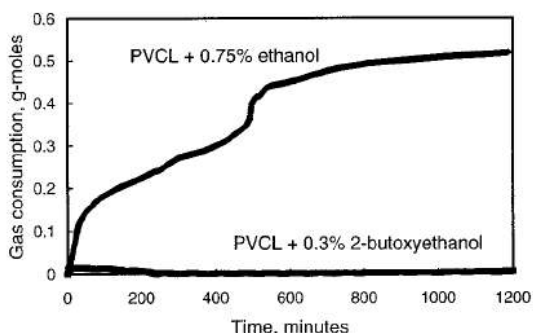
Fig. 6 Gas consumption comparison for PVCap plus ethanol (0.75wt%) versus 2-butoxyethanol (0.3wt%) measured at 4 °C, 1000 psig in 3.5wt% sea saltwater (reproduced with permission from ref. 66 )
