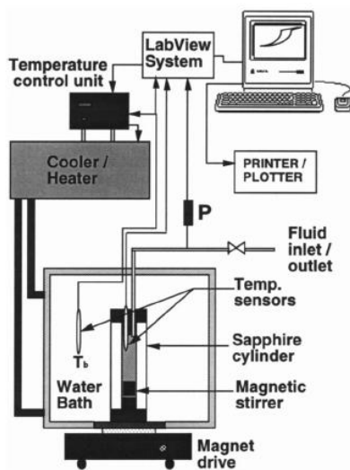
Fig. 5 Sapphire Cell Testing equipment (reproduced with permission from ref. 30 )
