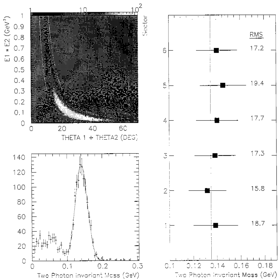
Fig. 17. Top Left: Distribution of E_1 * E_2 versus opening angle of 2 neutral hits detected in EC. Curves show constant invariant mass ( M^2 = 2 E_1 E_2 (1 - \cos \theta_{12}) ) for 2 photon decay of particle having masses 0.1 and 0.2 GeV. Bottom Left: Gaussian fit to measured \pi^0 invariant mass. Right: Sector dependence of \pi^0 invariant mass where both photons detected in same sector. RMS resolution displayed as error bars and listed at right in units of MeV.
