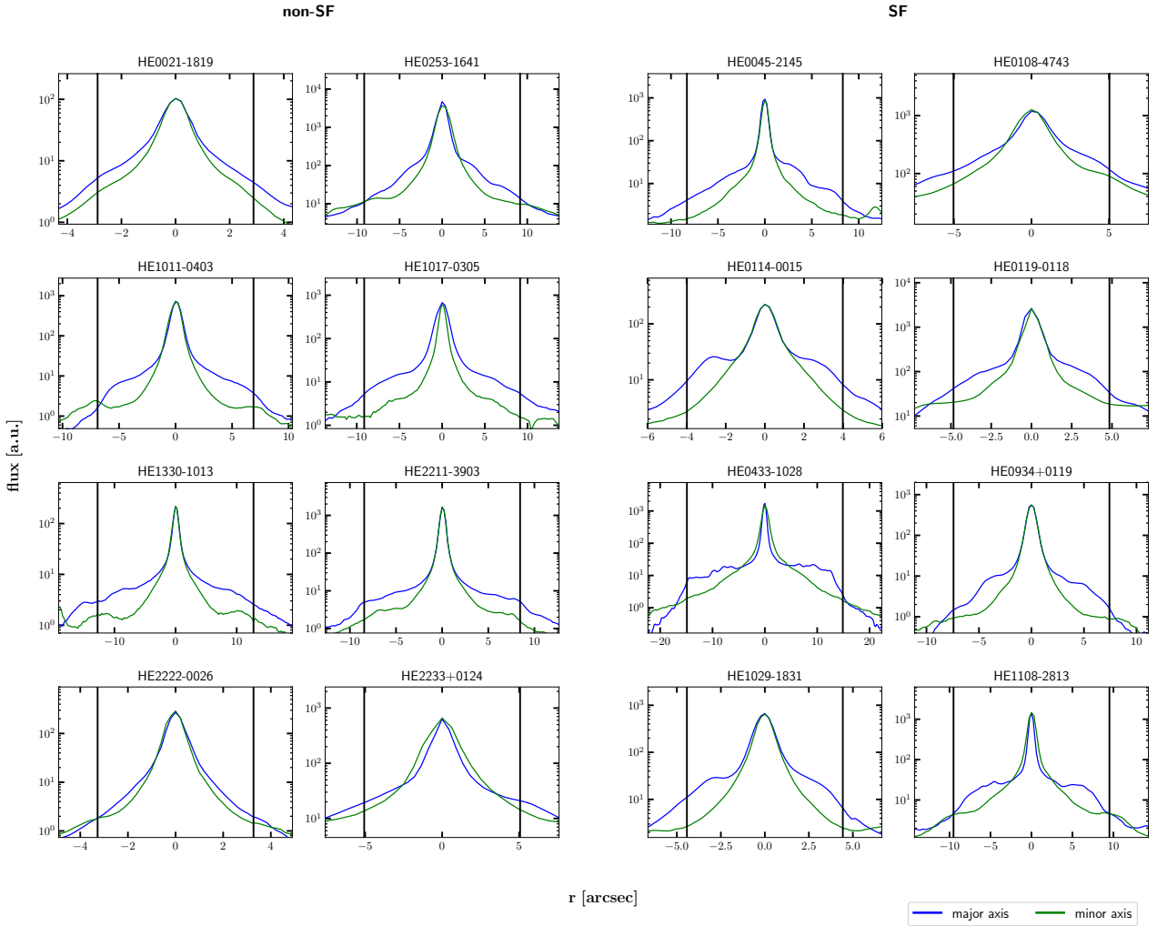
Fig. B.1. Radial surface brightness profiles along the major (blue) and minor (green) axes of the bar and continued into the disc. The distance on the x-axis is deprojected and scaled to the galaxy plane. The length of the bar is denoted by vertical black lines.
