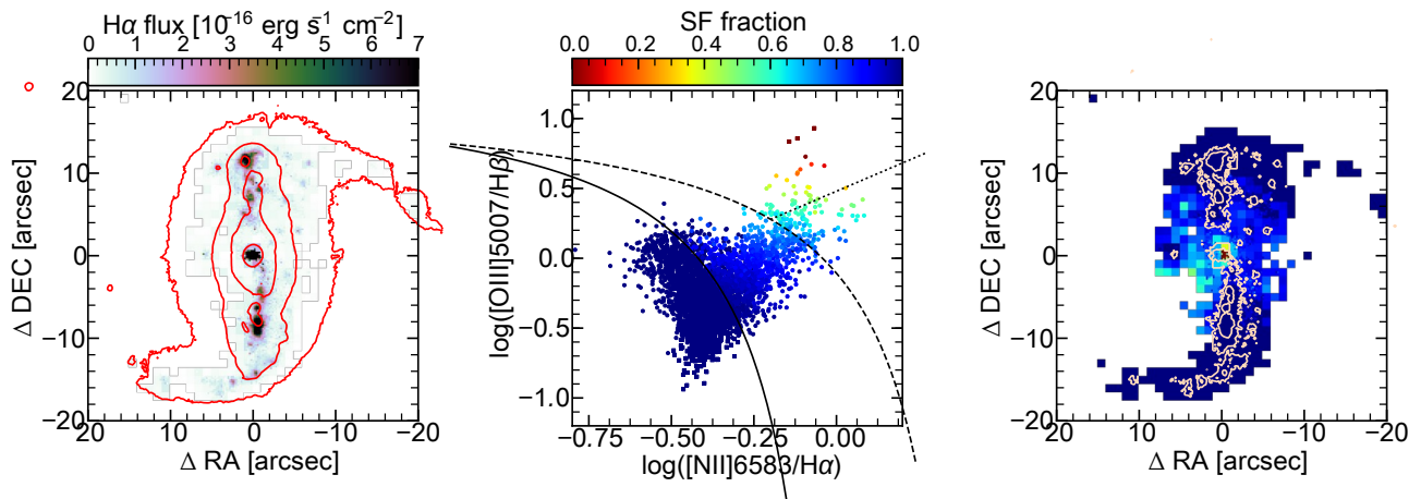
FIGURE 2. Left: AGN subtracted and extinction corrected H \alpha flux map, that traces the star formation in the galaxy with high resolution. i -band continuum emission is overlaid in red contours. The H \alpha emission shows an elongated distribution since the star formation regions are mostly situated within the stellar bar. Middle: Optical BPT-diagram (with division lines from Kewley et al. 2001; Kauffmann et al. 2003; Cid Fernandes et al. 2010) showing the ionization mechanisms of the nebular gas on a spaxel-to-spaxel basis. The AGN fraction is color-coded with red being purely excited by AGN and blue purely by star formation. Right: Map of the AGN fraction, with H \alpha contours overlaid. The flux in each pixel of HaMap is lowered by the respective AGN fraction to resemble the extended emission based on star formation.
