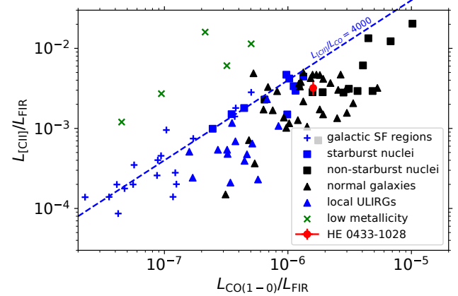
FIGURE 5. Position of HE0433-1028 in the L_{\text{CO}(1-0)} / L_{\text{FIR}} – L_{[\text{C II}]} / L_{\text{FIR}} plane compared to datapoints for normal galaxies, ULIRGs, galactic star formation regions, galactic nuclei, and low-metallicity galaxies from Stacey et al. (2010) and De Breuck et al. (2011) (and references therein). A typical starburst [C II]/CO line ratio of \sim 4000 is indicated.
