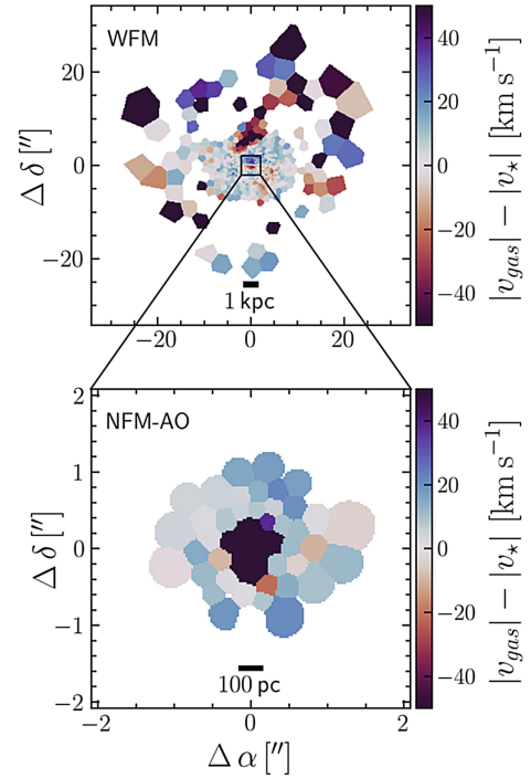
Fig. 9. Difference between Mrk 1044's gas and stellar velocity field from MUSE WFM ( top ) and NFM-AO ( bottom ). Except for the high velocity bloom that stretches \sim 5'' – 15'' north from the center, the gas rotates faster than the gravitationally driven motion of the stellar component.
