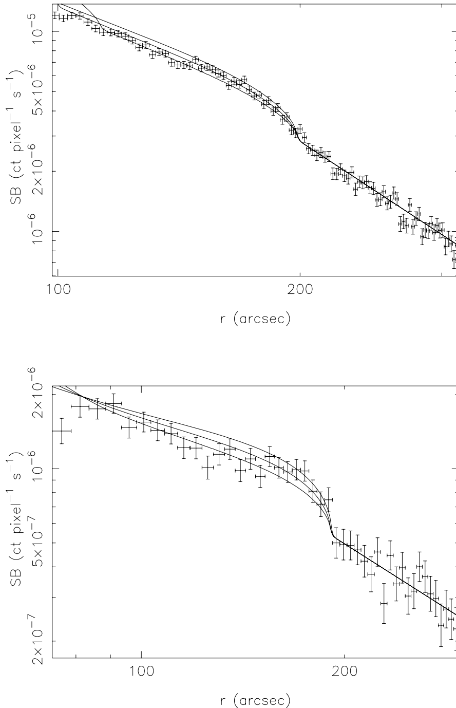
FIG. 3.—Surface brightness profiles of the shock front in Hydra A. Top : Radial surface brightness profile measured in the sector from P.A. 240^\circ to 300^\circ , to the west of the AGN, and in the energy range 0.6–7.5 keV. Surface brightness errors are 1\sigma statistical errors. Radial error bars show the limits of the bins. The smooth curves show surface brightness profiles for shock models with Mach numbers of 1.15, 1.19, and 1.23, from bottom to top. Models are scaled to match the observed surface brightness outside the shock. Bottom : Surface brightness profile at 0.6–7.5 keV of the shock front in the northeast, measured in a sector from P.A. 20^\circ to 50^\circ and centered 2.9 north of the AGN. Models are shown for shocks with Mach numbers of 1.26, 1.34, and 1.42.
