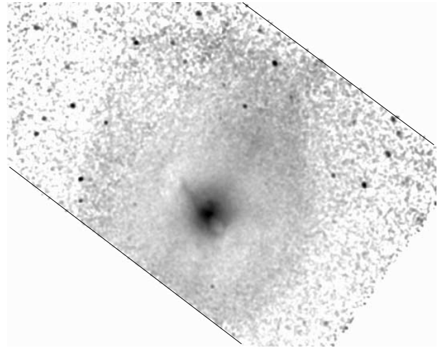
FIG. 1.— Chandra 0.5–7.5 keV image of Hydra A. The image from the S2 and S3 chips has been background-subtracted, exposure-corrected, smoothed with a 2'' Gaussian, and divided by a spherical beta model centered on the AGN. The distance between the edges of the chips (marked by lines running from northeast to southwest across the image) is 8.4' . The cavities of McNamara et al. (2000) can be seen close to the bright AGN. The cavity 1'-2' northeast of the AGN (cavity C), at the end of the bright filament, occurs where the 330 MHz radio jet bends sharply to the northwest (see Fig. 2). The shock front surrounding the radio lobes of Fig. 2 is visible, particularly to the east and north.
