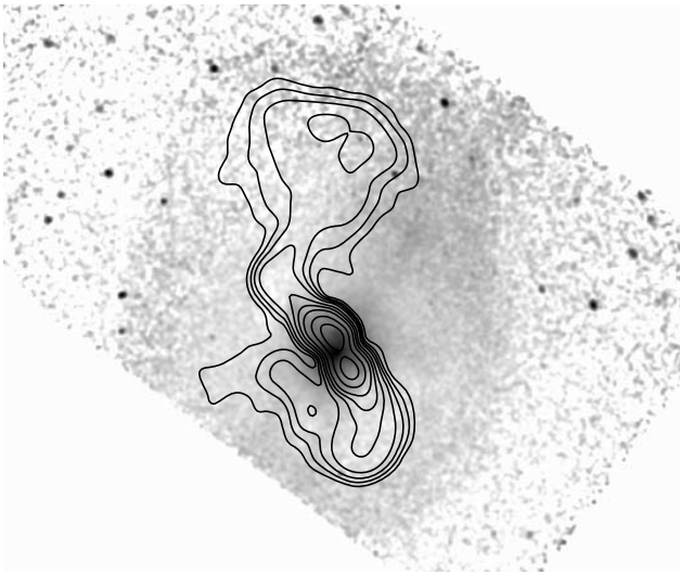
FIG. 2.—X-ray image of Hydra A with 330 MHz radio contours. The image of Fig. 1 is shown with logarithmically spaced contours from the 330 MHz radio map. The two closed contours near the center of the map are at the position of the 1.4 GHz radio lobes, marking the locations of the inner X-ray cavities that can be seen in Fig. 1.
