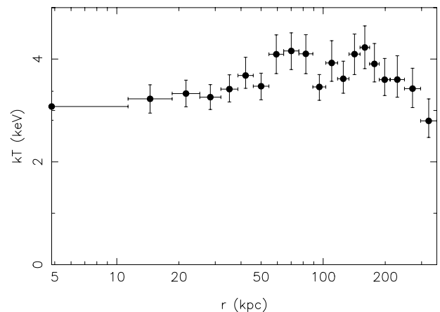
FIG. 5.—Western temperature profile of Hydra A, showing the projected temperature vs. radius in the sector from P.A. 240^\circ to 300^\circ . Error bars show 90% confidence ranges for the temperature.
