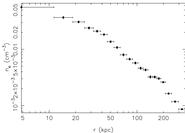
FIG. 4.—Western electron density profile of Hydra A, showing the deprojected electron density vs. radius in the sector from P.A. 240^\circ to 300^\circ . The shock jump is at 211 kpc. Density error bars are 90% confidence ranges, but some are hidden by the data point.
