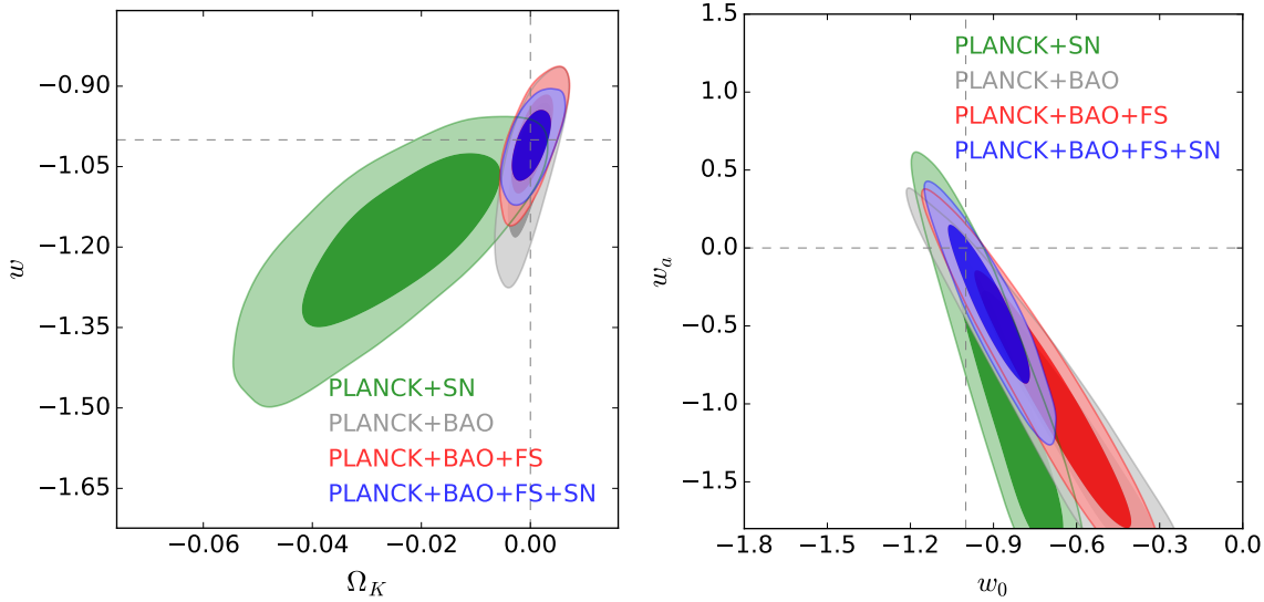
Figure 17. Parameter constraints for the \omega w CDM (left) and w_0 w_a CDM (right) cosmological models, comparing the results from BAO and BAO+FS to those with JLA SNe. One sees that the galaxy clustering results are particularly strong in the \Omega_K-\omega space and are comparable to the SNe in the w_0-w_a space.
