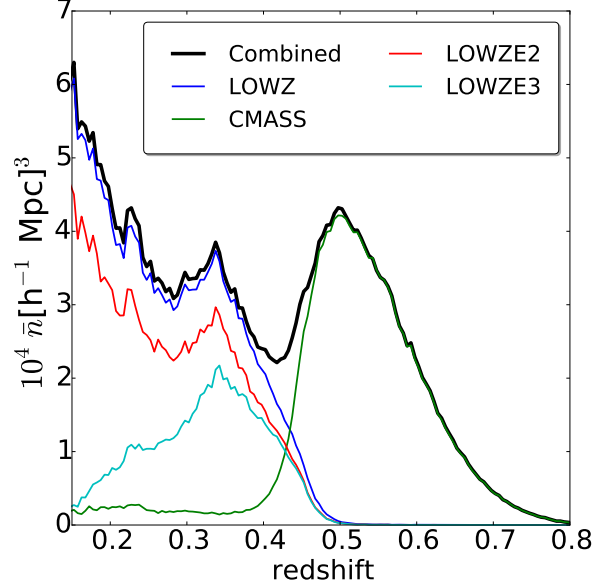
Figure 2. Number density of all four target classes assuming our fiducial cosmology with \Omega_m = 0.31 , along with the sum of the CMASS and LOWZ number densities (black).
