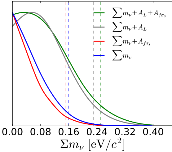
Figure 19. Posterior distribution for the sum of the mass of neutrinos in the \Lambda CDM cosmological model. The blue curve includes the growth measurement from the lensing impacts on the CMB power spectrum and from the BOSS RSD measurement of f\sigma_8 . The green curve exclude both of these constraints; one still gets constraint on the neutrino mass from the impact on the distance scale. Red and grey curves relax one of the growth measurements at a time; showing that most of the extra information comes from the CMB lensing. The vertical dashed lines indicate the 95% upper limits corresponding to each distribution.
