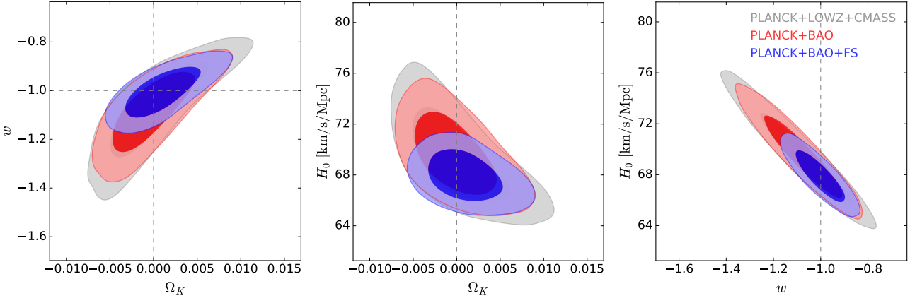
Figure 16. Parameter constraints for the \omega w CDM cosmological model, comparing the BAO and BAO+FS results from this paper as well as the DR12 LOWZ+CMASS results from Cuesta et al. (2016a). One sees that adding a 3rd redshift bin has improved the constraints somewhat, but full-shape information, especially the constraint on H(z)D_M(z) from the Alcock-Paczynski effect on sub-BAO scales, sharpens constraints substantially.
