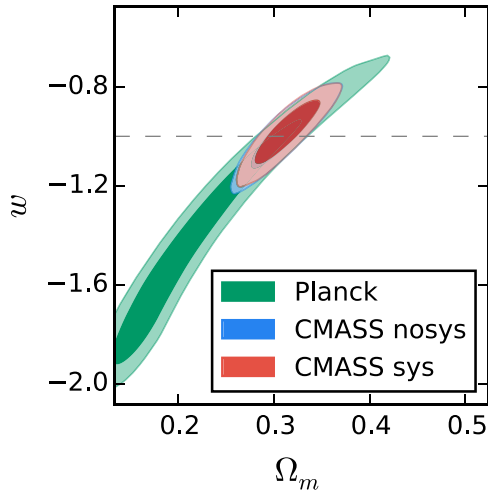
Figure 4. 2D marginalized contours for 68 per cent and 95 per cent confidence level for \Omega_m and w ( w CDM model assumed) from Planck -only (green), Planck +CMASS (red), and Planck +CMASS without including systematics weights (blue). One can see that w is consistent with -1 which is corresponding to the \Lambda CDM.
