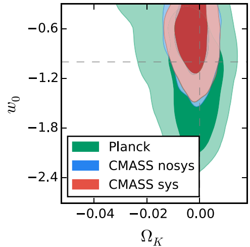
Figure 7. 2D marginalized contours for 68 per cent and 95 per cent confidence level for \Omega_K and w_0 ( w_0w_a CDM model assumed) from Planck -only (green), Planck +CMASS (red), and Planck +CMASS without including systematics weights (blue). One can see that \Omega_K and w_0 are consistent with 0 and -1 , respectively which are corresponding to the \Lambda CDM.
