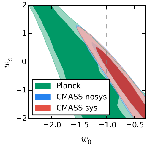
Figure 6. 2D marginalized contours for 68 per cent and 95 per cent confidence level for w_0 and w_a ( w_0w_a CDM model assumed) from Planck -only (green), Planck +CMASS (red), and Planck +CMASS without including systematics weights (blue). One can see that w_0 and w_a are consistent with -1 and 0, respectively which are corresponding to the \Lambda CDM.
