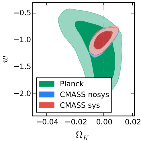
Figure 5. 2D marginalized contours for 68 per cent and 95 per cent confidence level for \Omega_K and w ( w CDM model assumed) from Planck -only (green), Planck +CMASS (red), and Planck +CMASS without including systematics weights (blue). One can see that \Omega_K is consistent with 0 and w is consistent with -1 which is corresponding to the \Lambda CDM.
