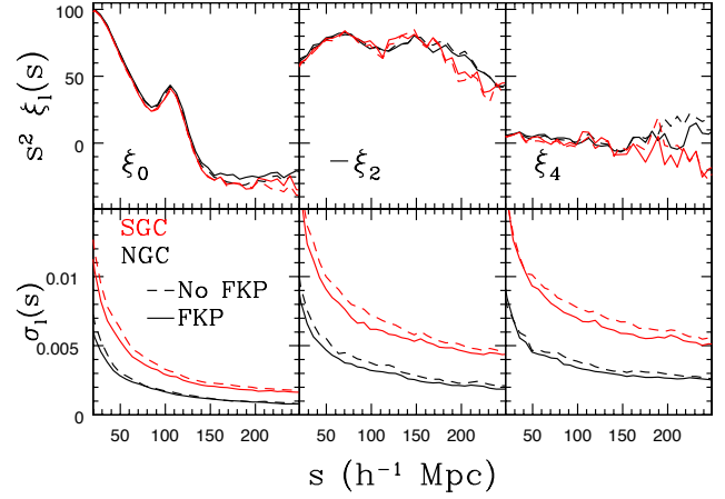
Figure 6. Top panels: The average of \xi_\ell(s) we determine using 600 mocks, for the NGC (black) and SGC (red) footprints and with (solid lines) and without (dashed lines) FKP weights. The baryon acoustic oscillation peak can clearly be seen at s \sim 100h^{-1}\text{Mpc} in \xi_0 . Bottom panels: the standard deviation of the 600 mocks, using the same scheme as the top panels.
