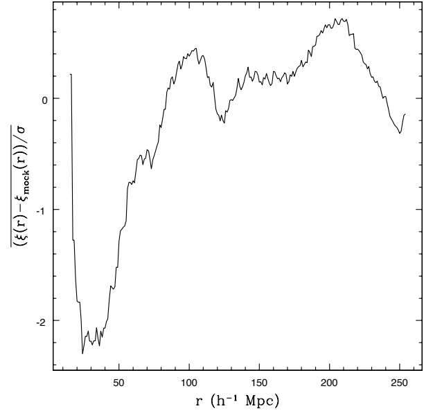
Figure 24. The average value of (\xi[r_{\parallel}, r_{\perp}] - \bar{\xi}_{mock}[r_{\parallel}, r_{\perp}])/\sigma calculated in rings with \Delta r = 10h^{-1} and (r - \Delta r)^2 < r_{\parallel}^2 + r_{\perp}^2 < (r + \Delta r)^2 .
