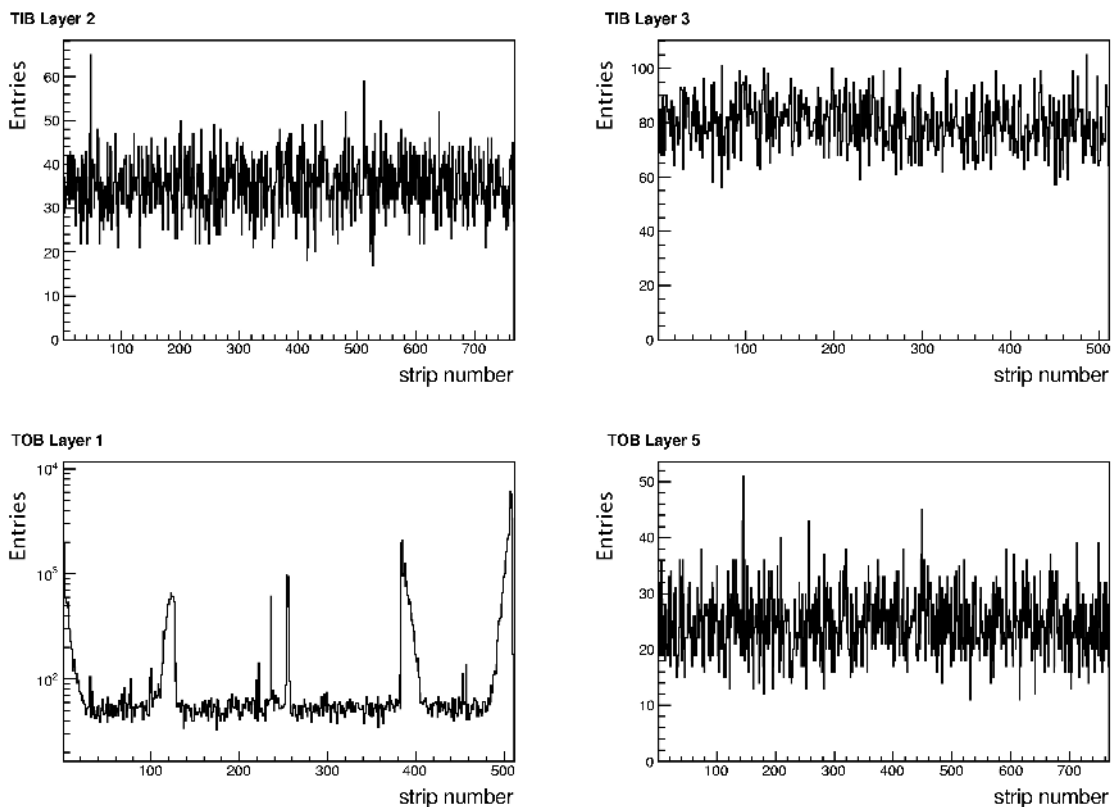
Figure 57. Cluster position for TIB and TOB at B = 0 T.
