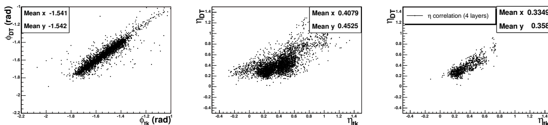
Figure 55. Correlations of directions of tracks, in the absence of magnetic field, reconstructed in the tracker and in the Drift Tubes. The \phi correlation is shown left. The \eta correlation for all the tracks (for tracks with hits in 4 layers) is shown in the centre (right).
