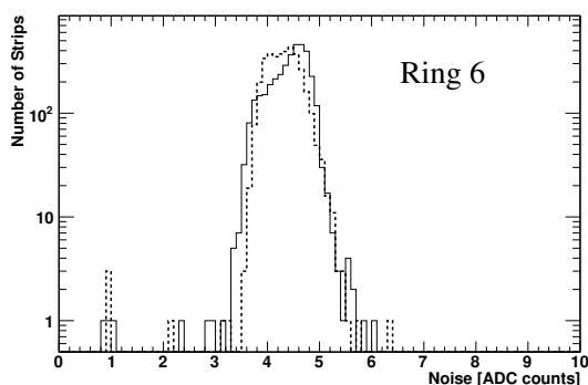
Figure 40. Tick mark height calibrated (dotted) and uncalibrated (solid) noise of ring 6 modules.
