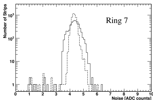
Figure 41. Tick mark height calibrated (dotted) and uncalibrated (solid) noise of ring 7 modules.
