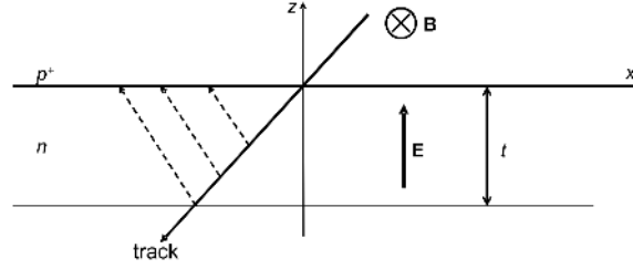
Figure 77. Lorentz drift in the microstrips silicon sensors.
